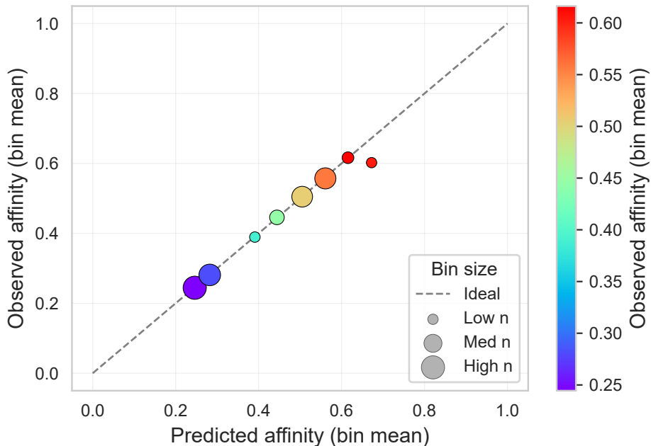
Reliability diagram (ECE=0.002, MCE=0.070)
