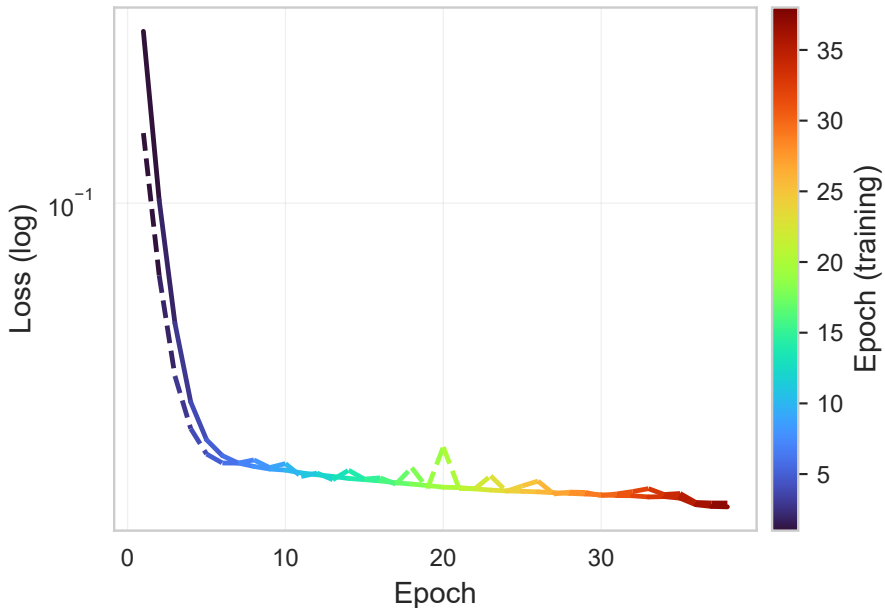
Model loss over epochs (turbo gradient; dashed = validation)
