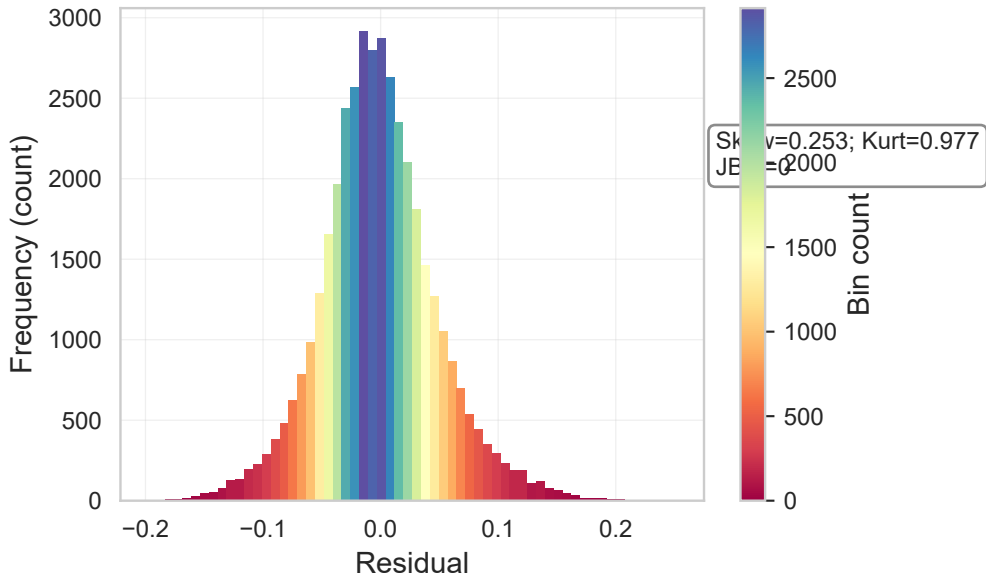
Distribution of residuals
