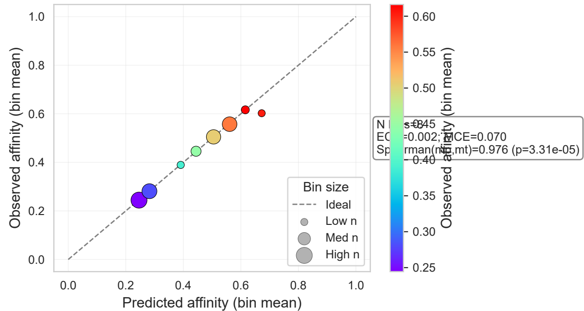
Reliability diagram
