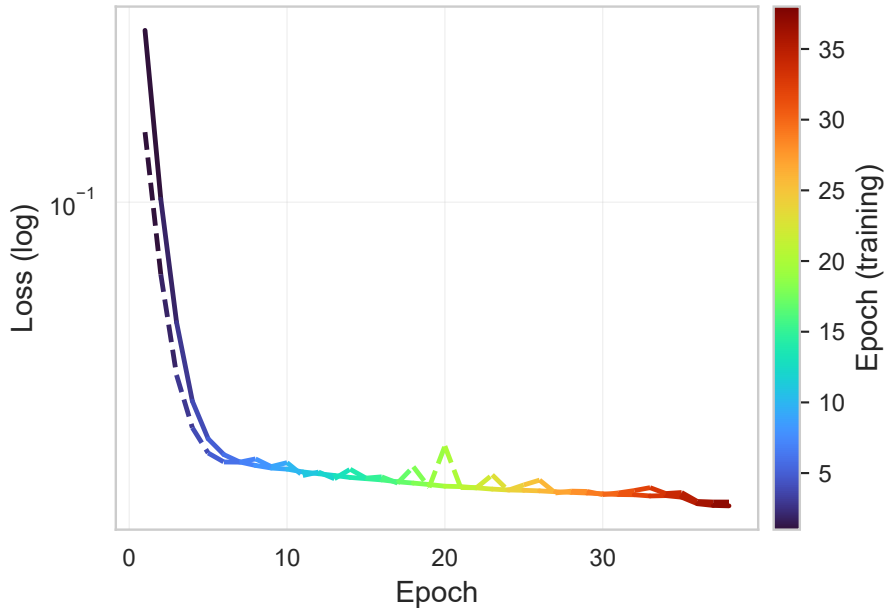
Model loss over epochs (turbo gradient; dashed = validation) — best val_loss=0.0157 @ epoch 38
