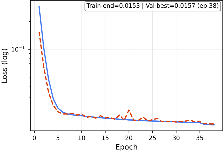
Model loss over epochs (dashed = validation) — best val_loss=0.0157 @ epoch 38
