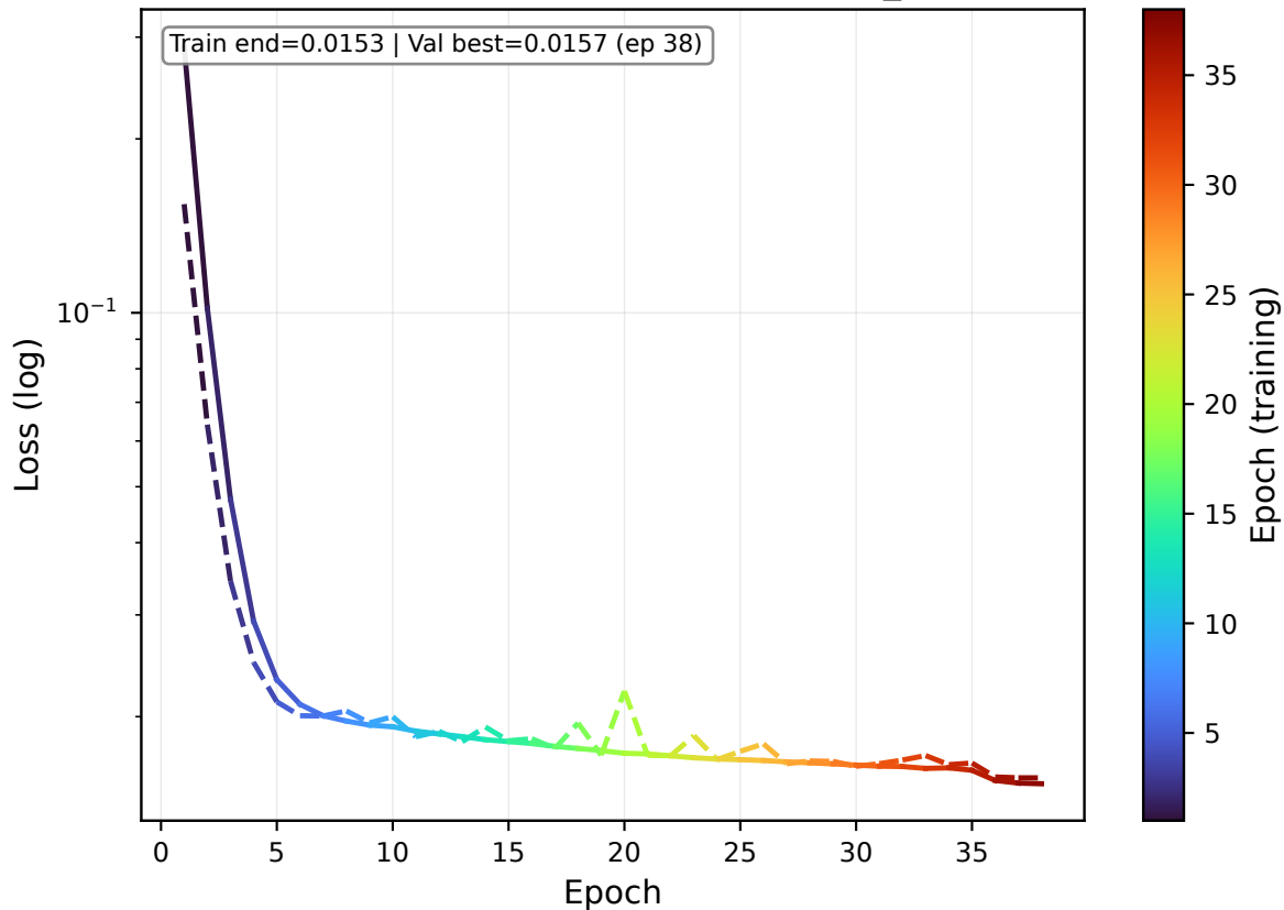
Model loss over epochs (dashed = validation) — best val_loss=0.0157 @ epoch 38
