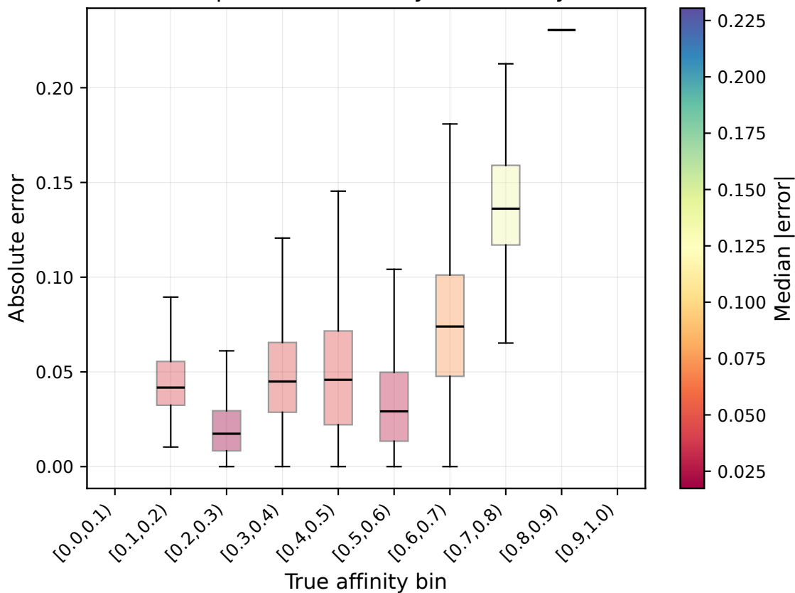
Absolute prediction error by true-affinity bins
