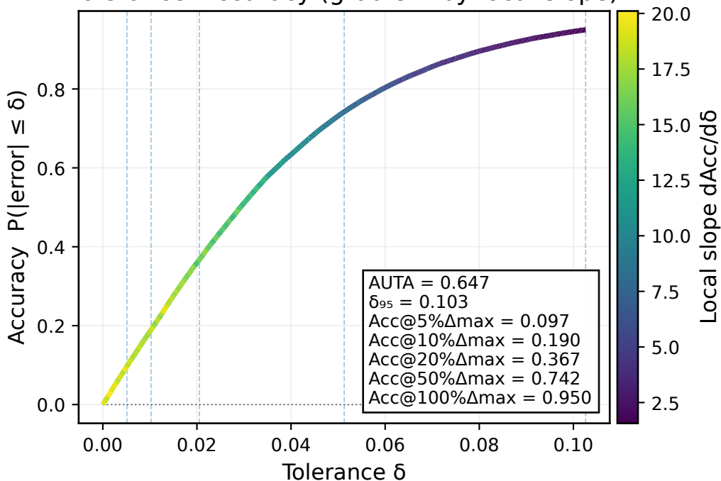
Tolerance-Accuracy (gradient by local slope)
