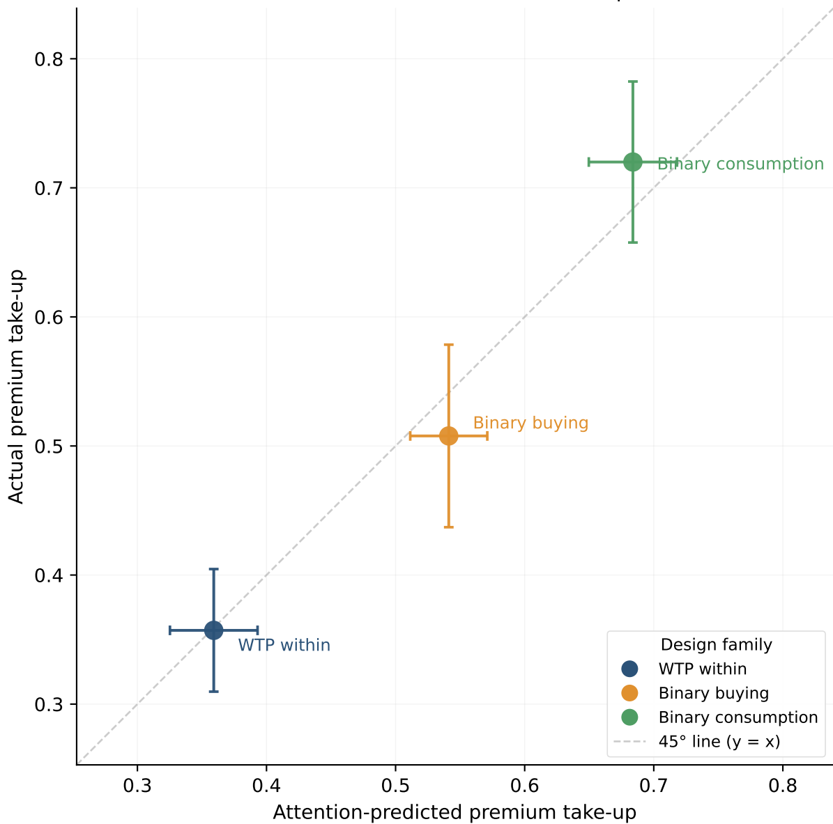
Actual versus Attention-Predicted Premium Take-up (Fine-Tuned LLM)
