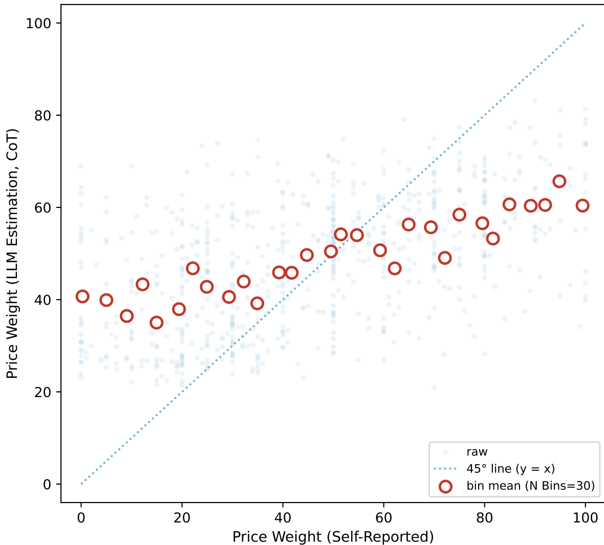
v5 (CoT) — LLM vs Self-Reported (Pearson r = 0.520^{***} )
