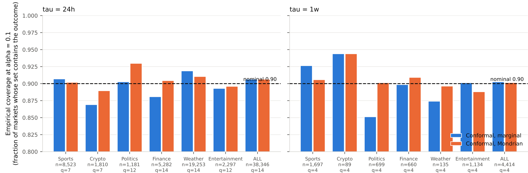
H2 — coverage at alpha = 0.1 by domain: one pooled threshold vs one threshold per domain
