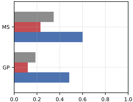
StudPerf: school
