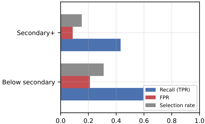
StudPerf: mother_edu
