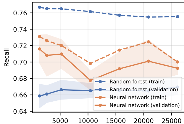
OULAD (week-4 features)
