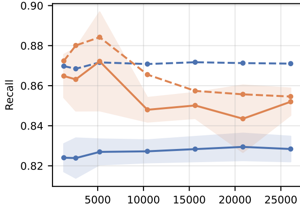
OULAD (full-module features)
