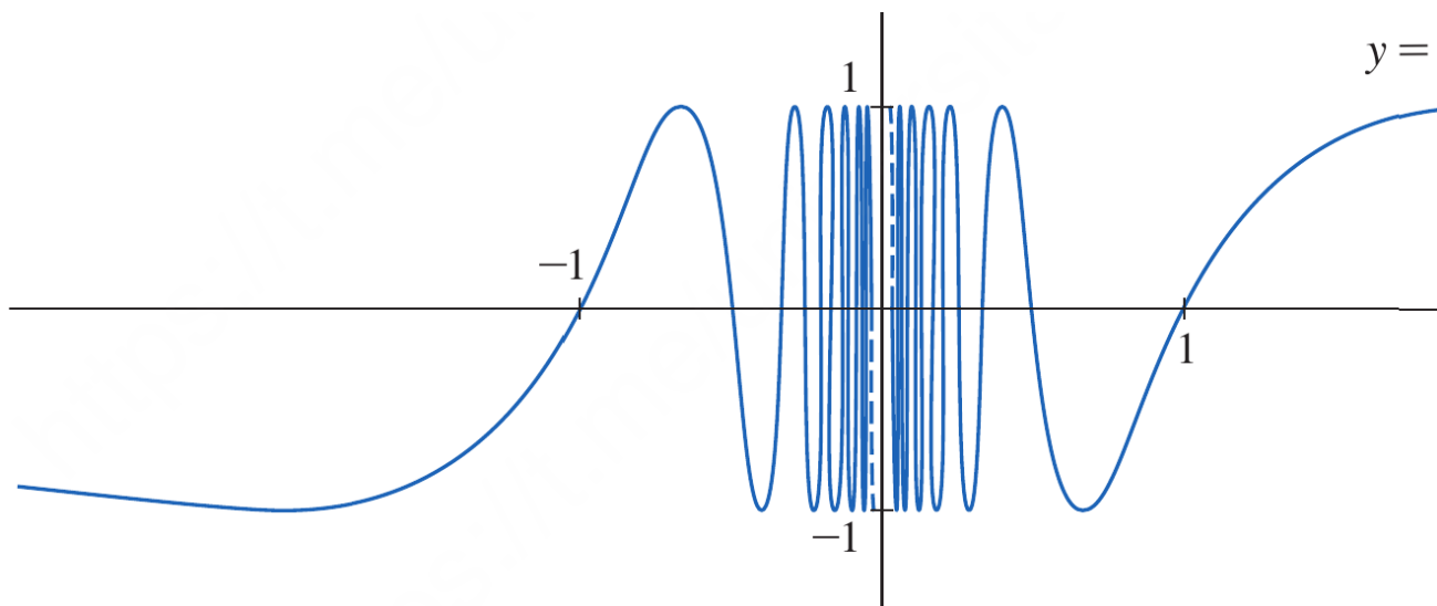
Figure 8.1. Graph of y = \sin(\pi/x) showing increasingly rapid oscillation near x = 0 .
