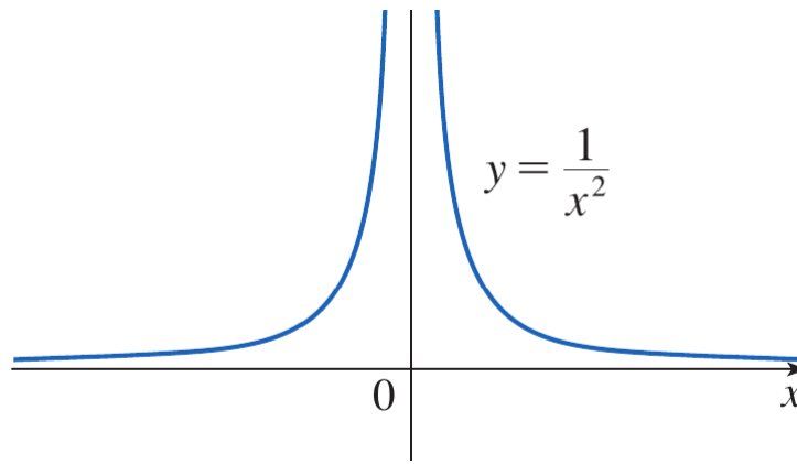
Figure 9. Graph of y = \frac{1}{x^2} showing unbounded behavior near x = 0 .
