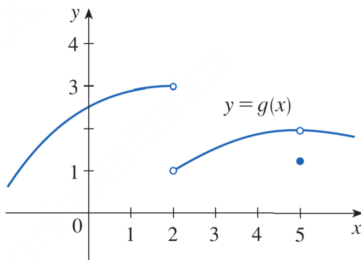
Figure 7. The graph of a function g .
