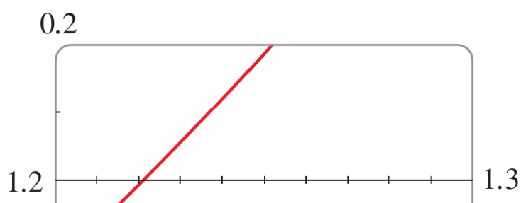
Figure 10. Graph of f(x) = 4x^3 - 6x^2 + 3x - 2 showing a zero between 1 and 2.
