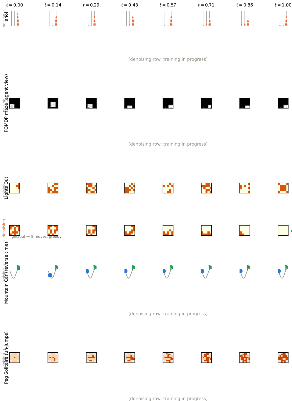
Figure 4: Noising and denoising, domains 6–10: Hanoi, POMDP maze (the strip shows the agent’s masked view), Lights Out, Mountain Car (reverse-time noising visible as the car being carried away from the flag), and Peg Solitaire (noising = \frac{1}{5} un-jumps that add pegs; denoising = jumps that remove them).
