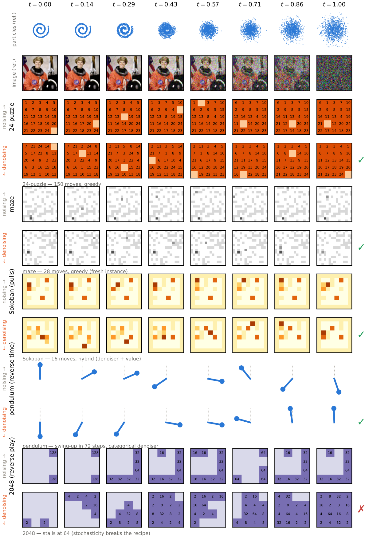
Figure 3: Noising and denoising, domains 1–5. 4 The two reference rows at the top show the same t grid on the classic diffusion visuals—a spiral particle cloud and a photograph under Gaussian noise—so each domain strip below reads as the same schedule with a different noise operator. Top
