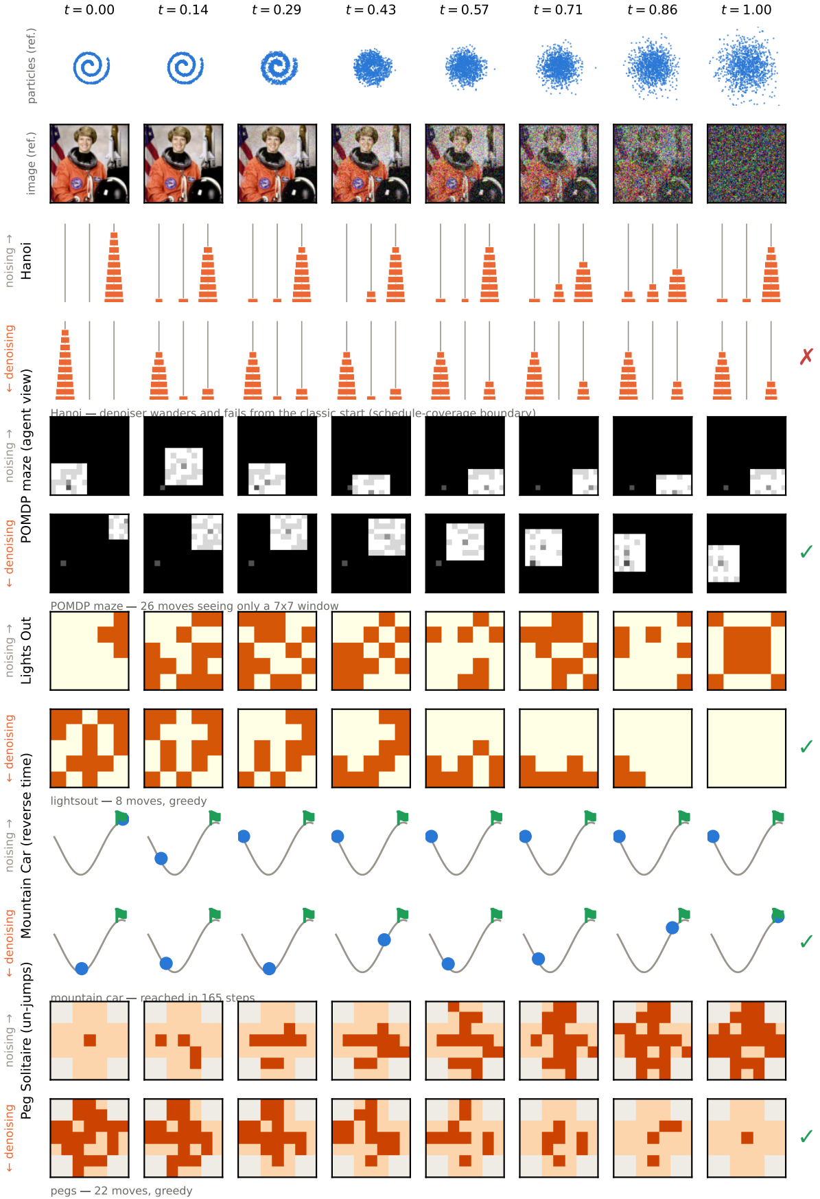
Figure 4: Noising and denoising, domains 6–10 ( 5 reference rows as in Fig. 3): Hanoi (the denoising row shows the trained denoiser wandering and failing from the classic all-on-one-peg start—the schedule-coverage boundary of §4.1 made visible), POMDP maze (the strip shows the agent’s schedule), Lights Out, Mountain Car (the denoising row is visible), and Peg Solitaire (the denoising row is visible).
