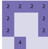
2048 (stochastic)
