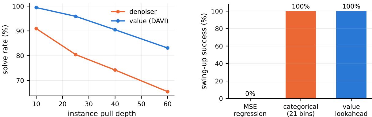
Figure 7: Left: Sokoban solve rate vs. difficulty; reverse-only training is deadlock-blind. Right: the pendulum ablation — \epsilon -regression collapses to the bimodal posterior’s mean; the same data with a 21-bin categorical head restores 100%.
