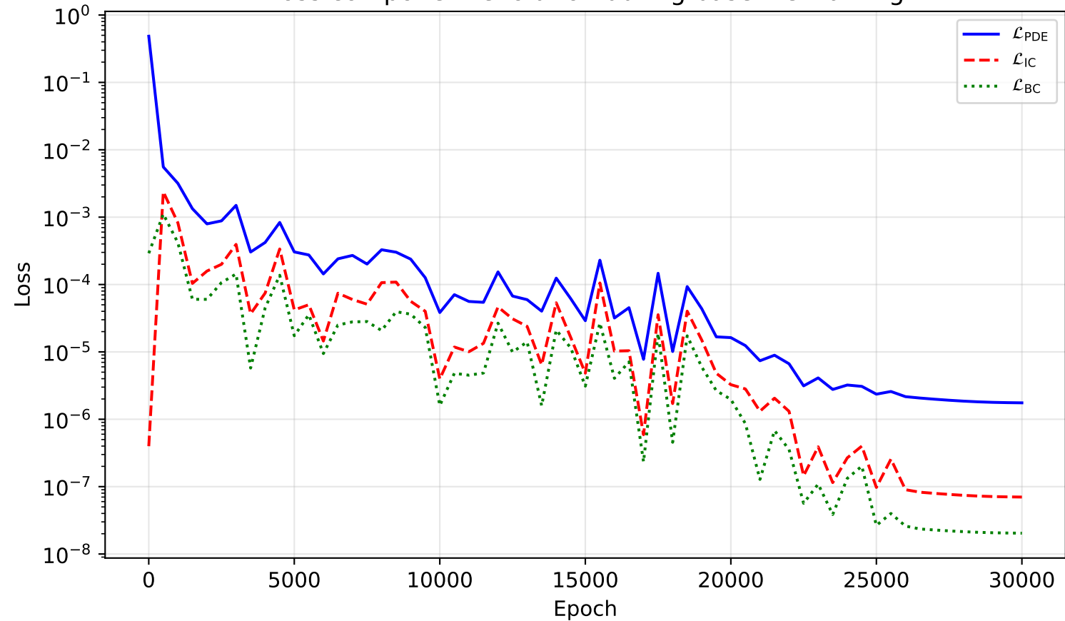
Loss component evolution during baseline training
