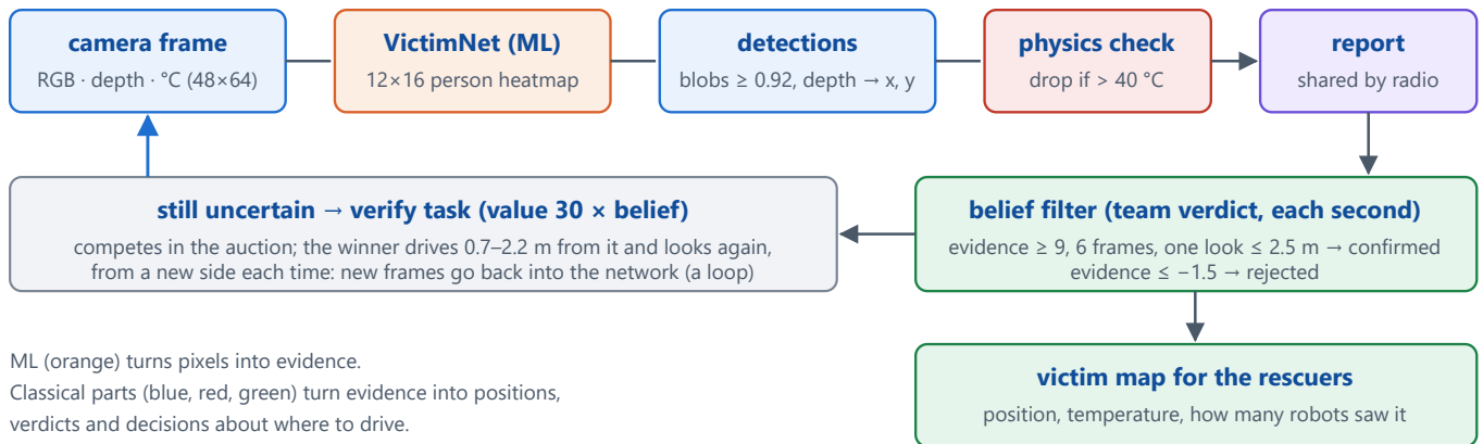
Figure 7.0 The whole ML pipeline, including the loop back: an uncertain sighting sends a robot for a closer look, and the new images go through the network again.
