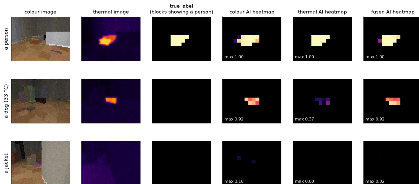
Figure 7.4 One person, one dog and one jacket, each seen from about 2 m, and what each detector makes of them (brighter = more likely a person; "max" is the highest block). All three are certain about the person. The jacket fools nobody here: it is cold, and its shape is wrong. The dog is the hard case. The thermal detector stays low (0.37), because the warm shape is too small. But the colour and fused detectors reach 0.92, exactly the detection threshold. Only repeated, close, confident looks can confirm such a sighting.
