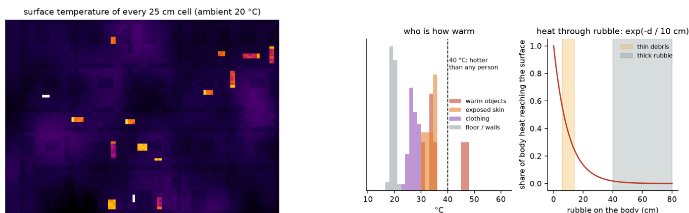
Figure 5.1 Left: the temperature field of an apartment block in the "ironbow" palette used by thermal cameras (black = cold, white = hot). Bodies, a dog and hot water glow; the walls are slightly cooler. Middle: the temperature ranges overlap. Clothing, skin, dogs and warm rubble share 28–36 °C, which is why temperature alone cannot identify a person. Right: how quickly rubble blocks heat.
