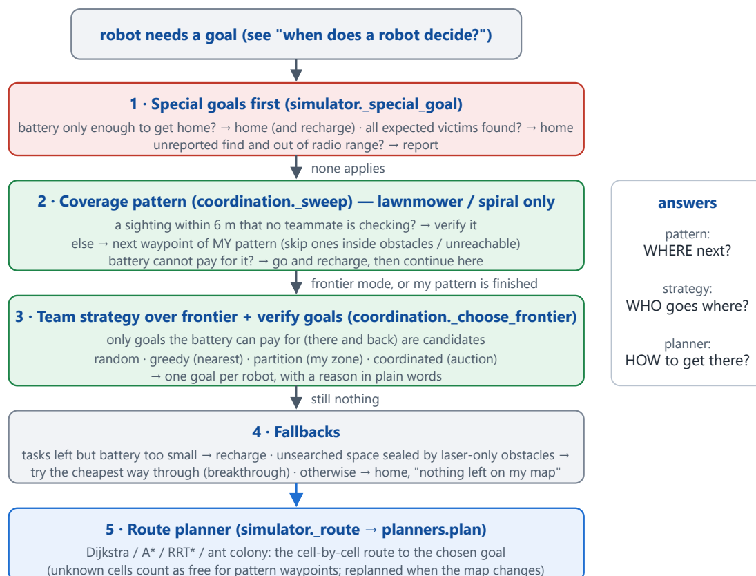
Figure 8.1 How one goal is chosen. The layers are tried top to bottom. The first layer that produces a goal wins, and the route planner then turns that goal into a route. This is Simulator._decide , which calls coordination.choose .
