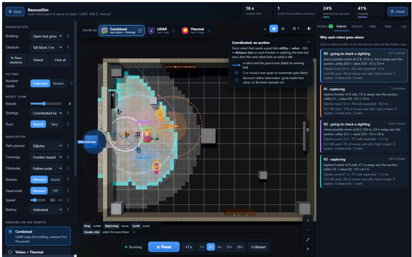
Figure 8.4b The strategy layer during a coordinated mission on the test ground (16 s). A line in each robot's colour runs to the goal it won, and the label above the goal is its winning bid. Around a won goal, the shaded 2 m circle is closed to teammates and the dashed ring marks the discount radius. With partition the layer draws each zone's border in its owner's colour instead; greedy goals have dashed lines, random goals dotted ones. The card top right explains the current strategy.
