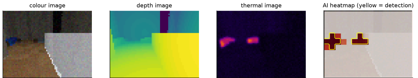
Figure 4.3 What one robot sees in one frame, all rendered by sensors.render : the colour image (headlamp only), the depth image (dark = near), the thermal image (two warm body parts glow), and the detector's heatmap on top (chapter 7). Yellow outlines are the blocks above the detection threshold.
