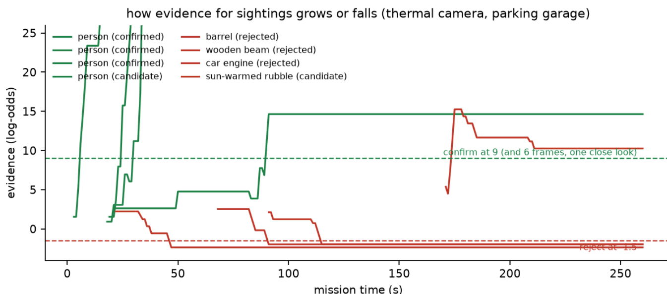
Figure 7.3 Evidence for sightings during one thermal mission. Green lines are real people: repeated close looks push them past 9 quickly. Red lines are other things: a barrel, a beam and a warm engine sink to the rejection line once robots look closely. One sun-warmed rubble pile rose above 9 but was not confirmed, because the other conditions (6 frames, a close look) were not met. That is exactly what they are for.
