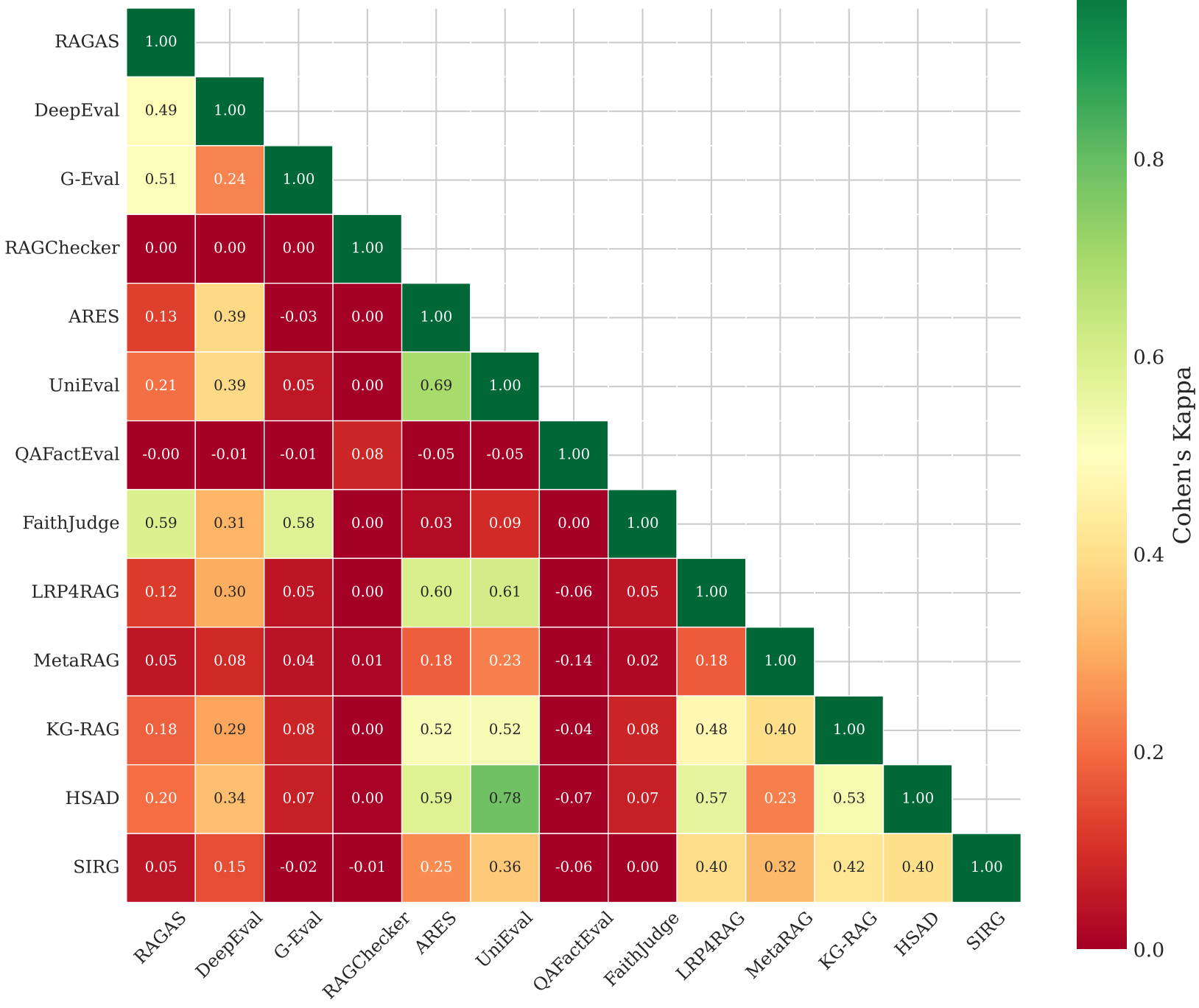
Cohen's Kappa (threshold=0.5)
