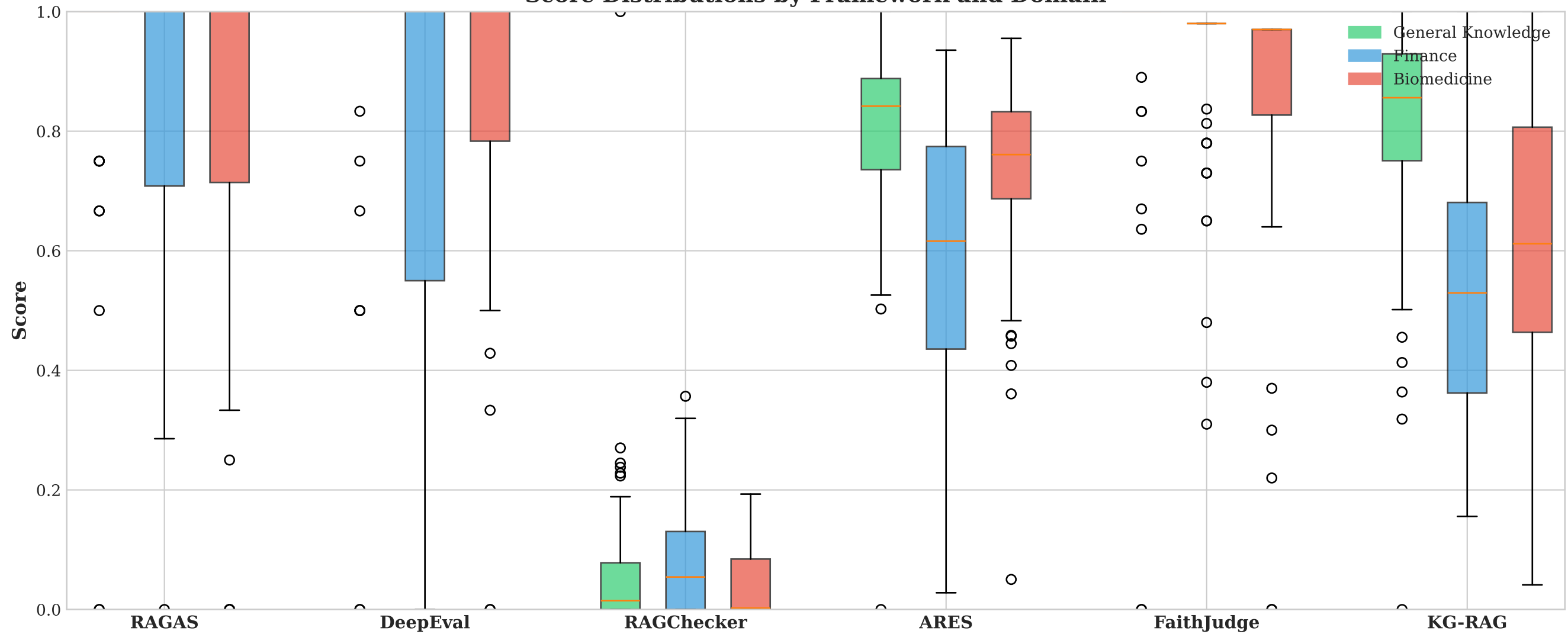
Score Distributions by Framework and Domain
