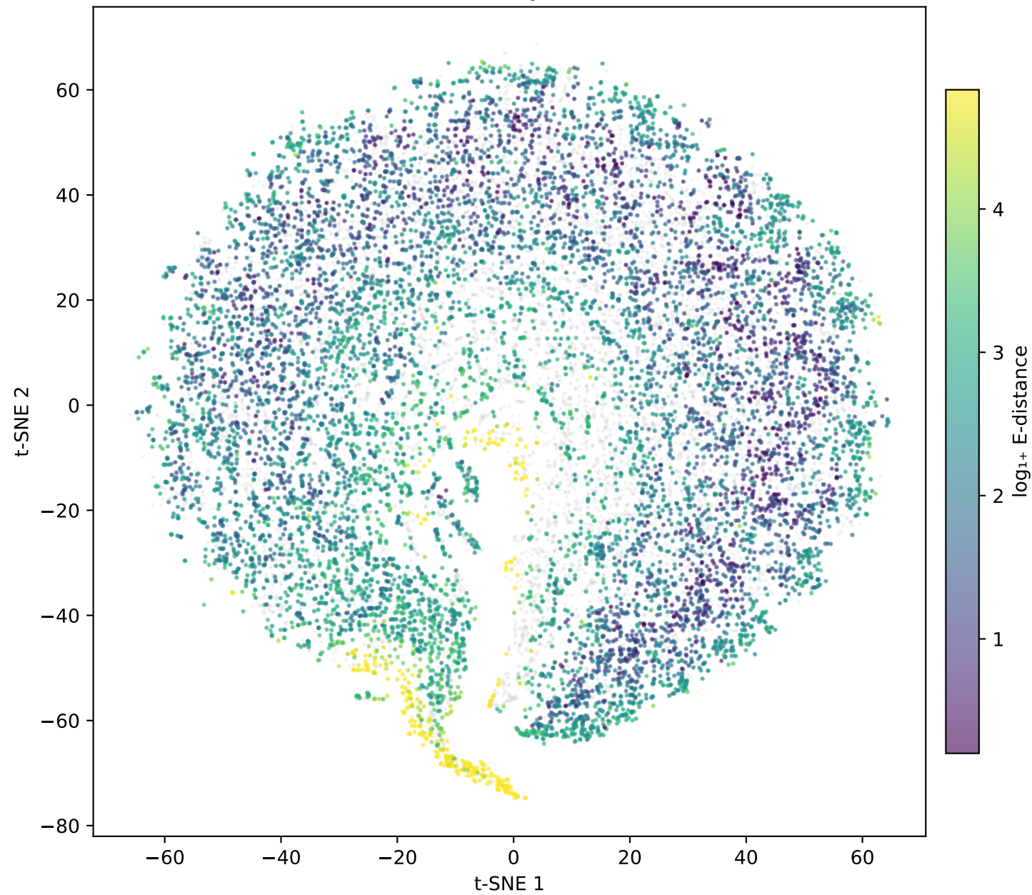
t-SNE colored by E-distance
