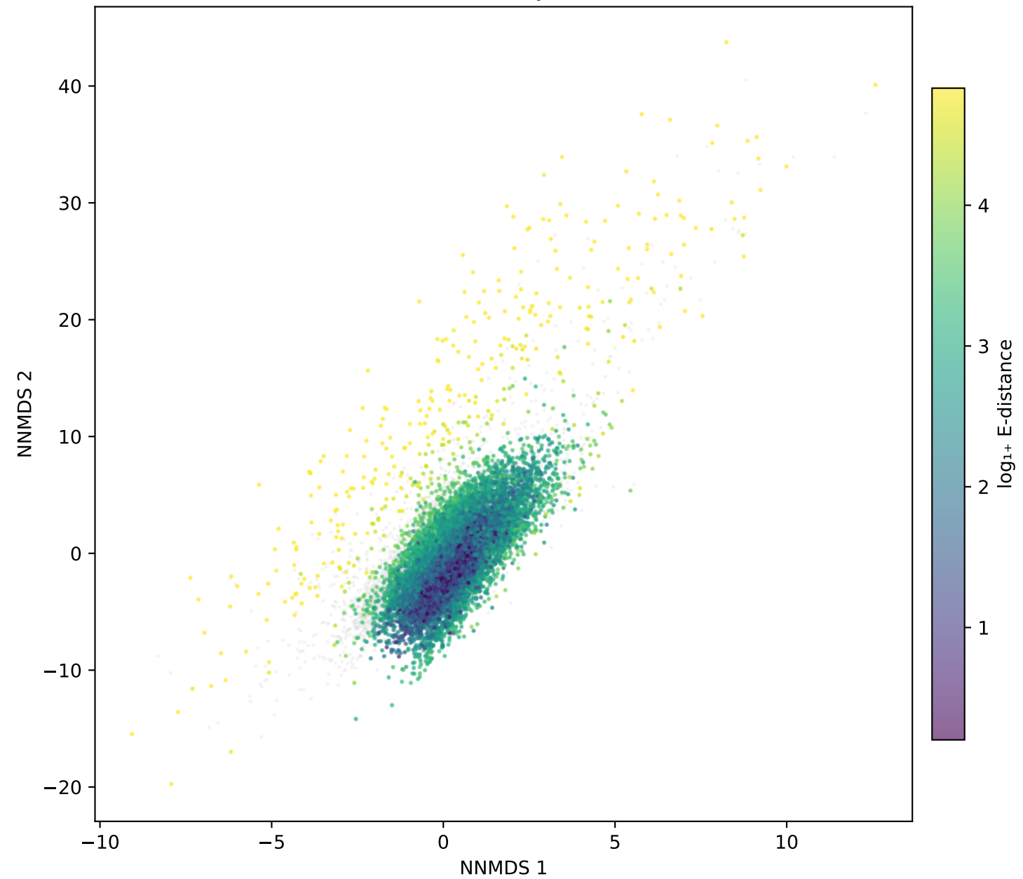
NNMDS colored by E-distance
