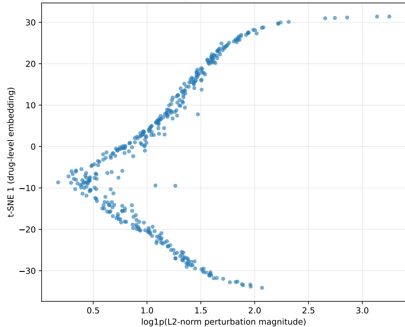
t-SNE1 vs Magnitude (Spearman r = 0.436 )
