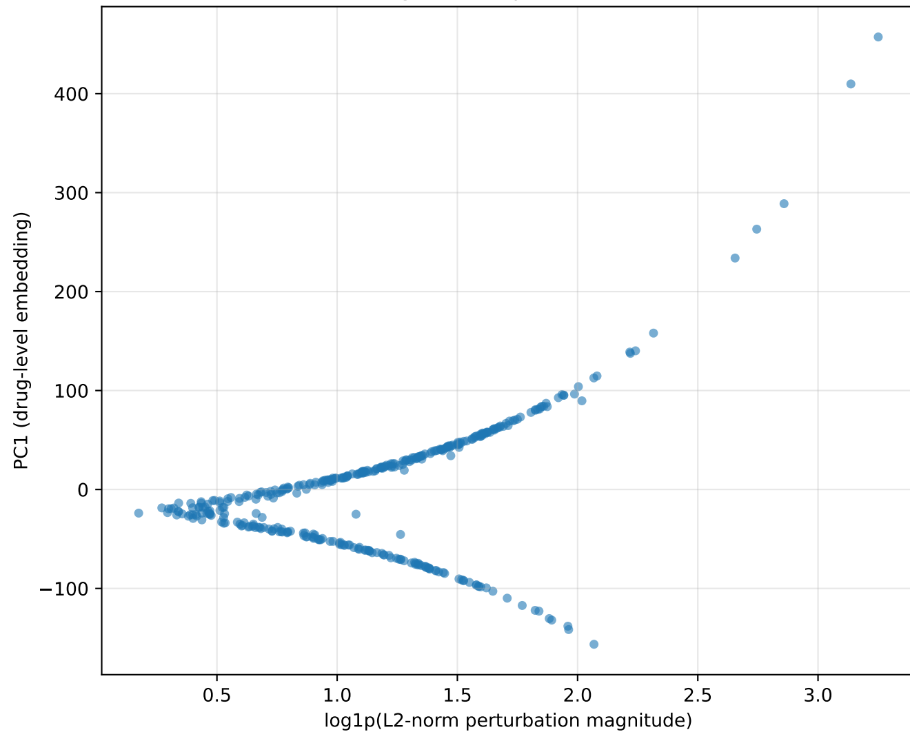
PC1 vs Magnitude (Spearman r = 0.436 )
