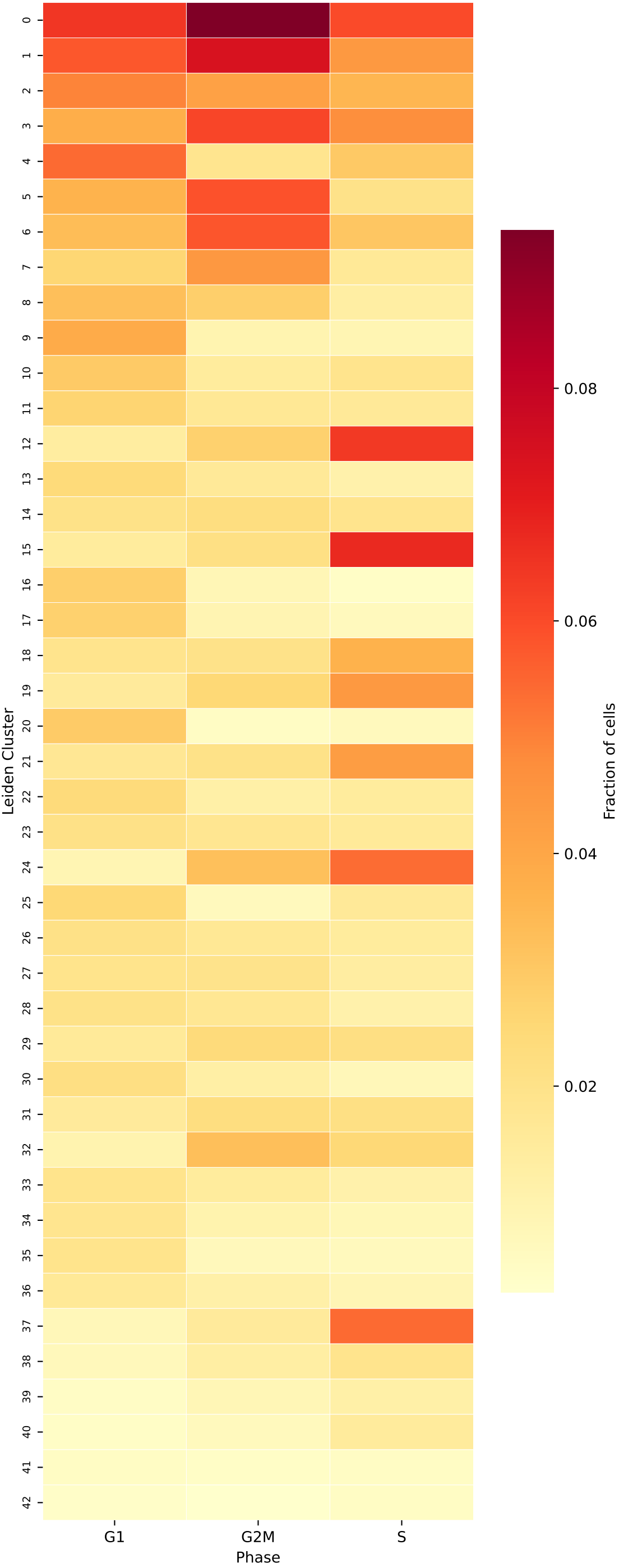
Leiden clusters vs Cell Cycle (lncRNA, res=0.5)
