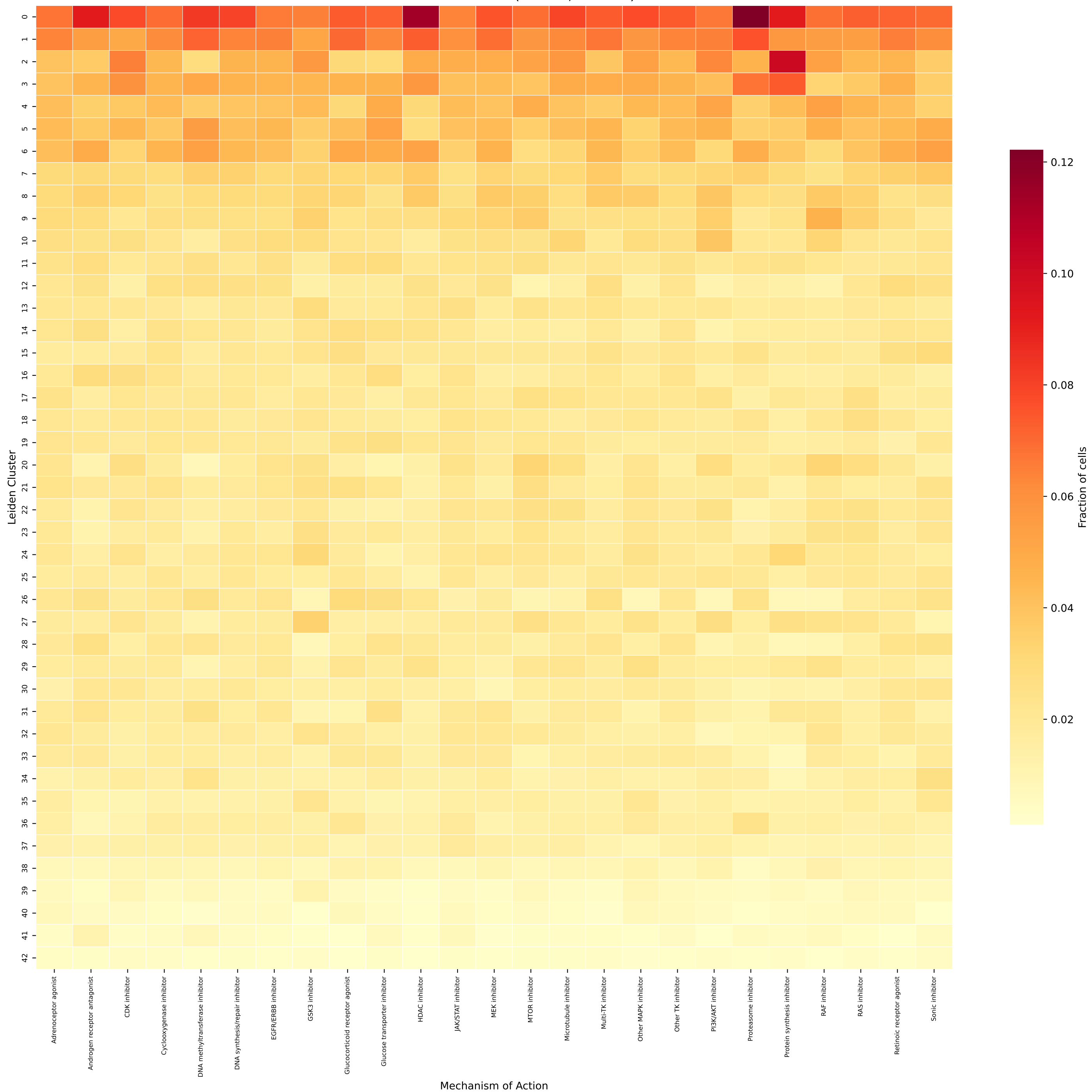
Leiden clusters vs MOA (lncRNA, res=0.5)
