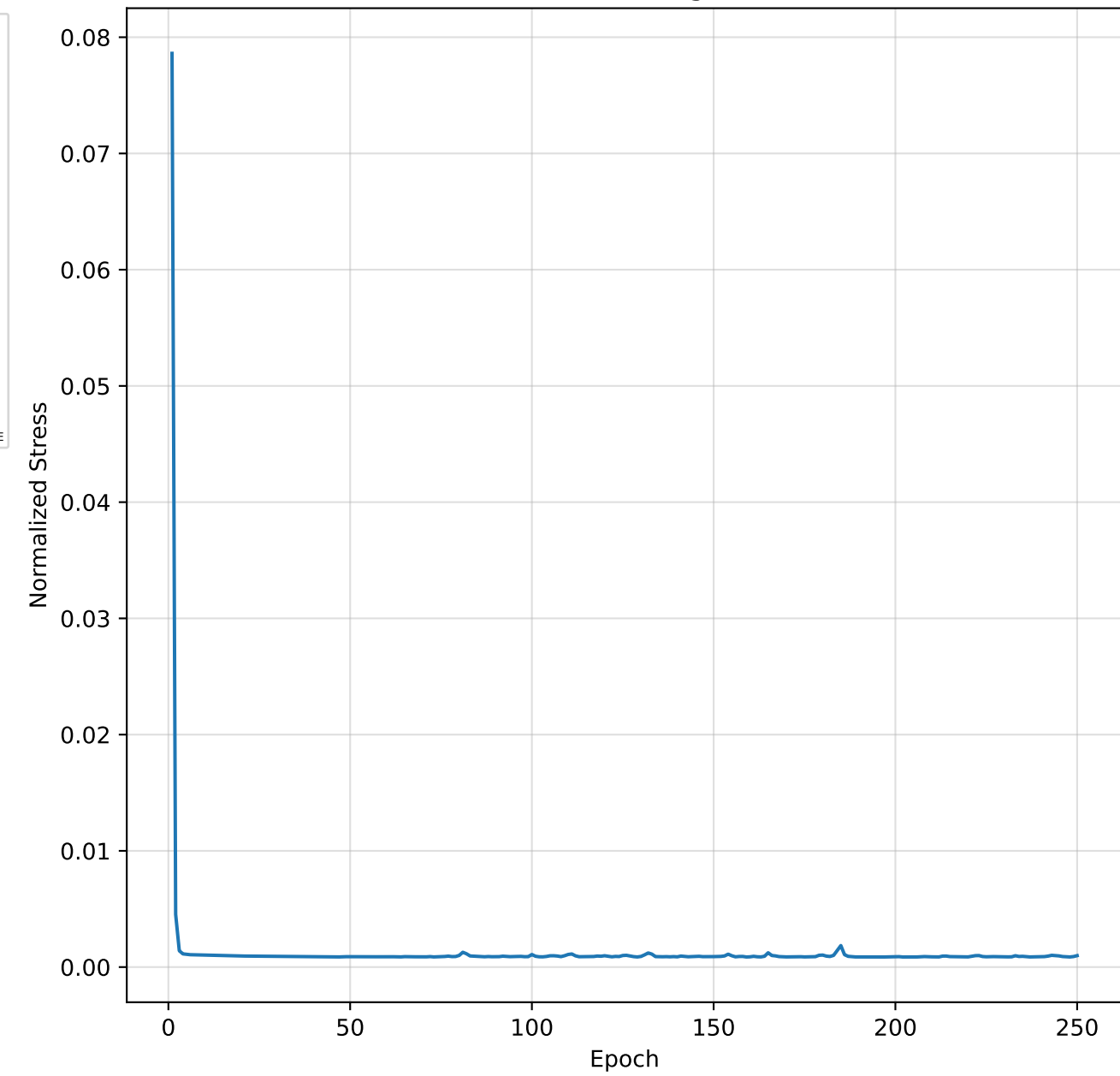
NNMDS Training Loss
