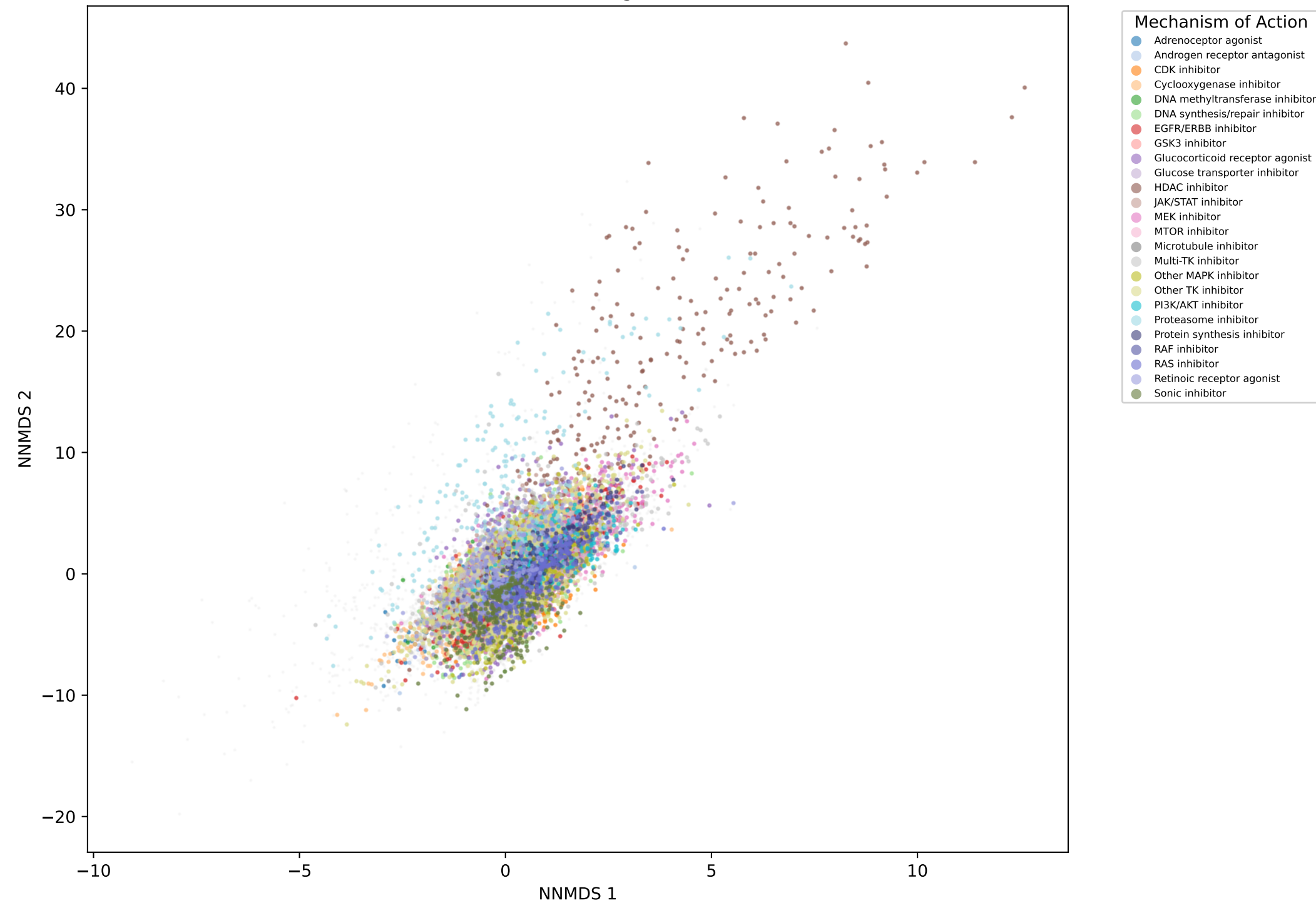
NNMDS — Drug MOA
