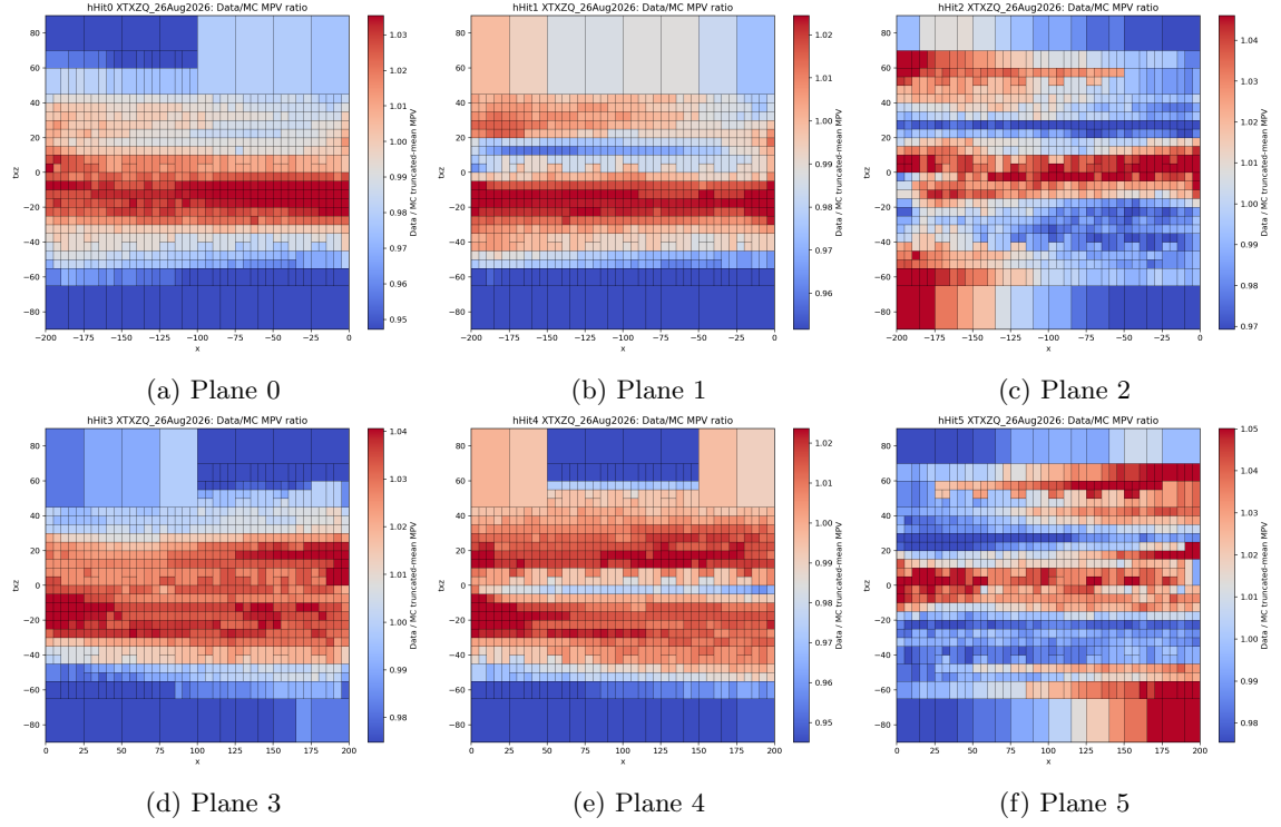
Figure 9: XTXZQ data/MC MPV ratio maps for all planes.
