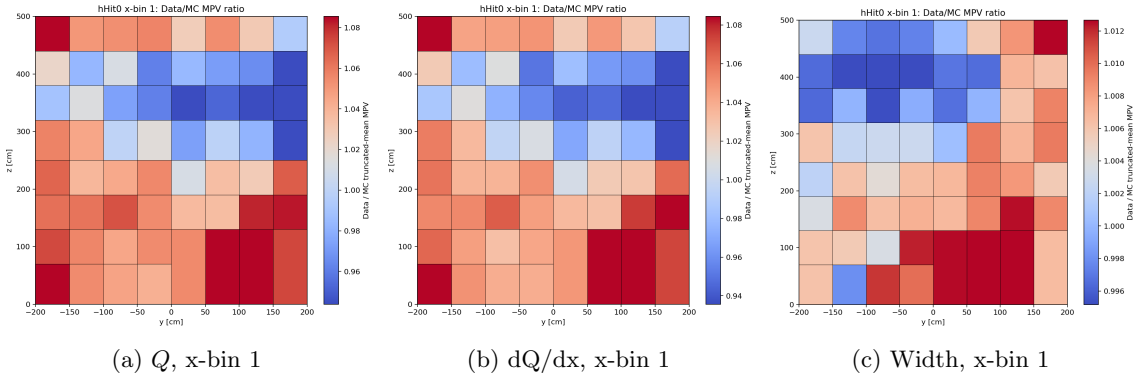
Figure 4: Example YZ data/MC MPV ratio maps for plane 0, angular region 001, and three response observables.
