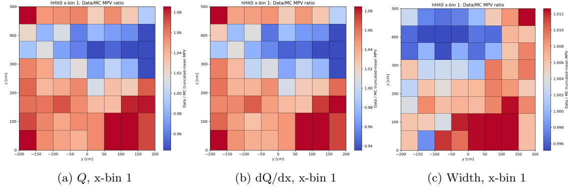
Figure 9: Example YZ data/MC MPV ratio maps for plane 0, angular region 001, and three response observables.
