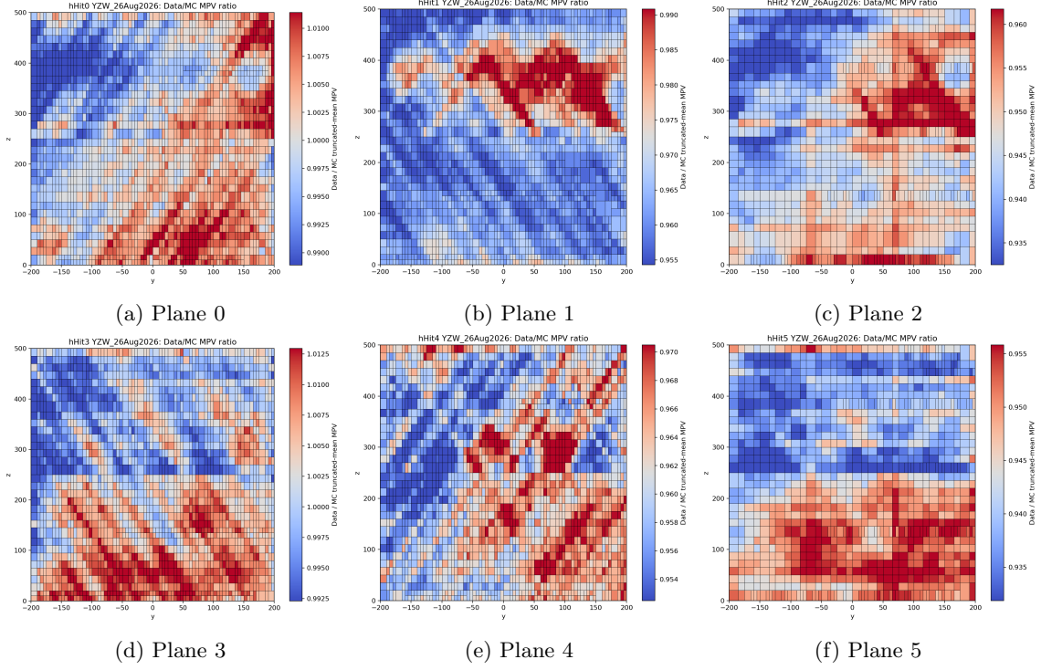
Figure 13: YZW data/MC MPV ratio maps for all planes.
