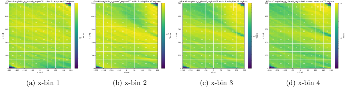
Figure 8: Example adaptive YZ regions for plane 0, angular region 001, in the first four x-bins.
