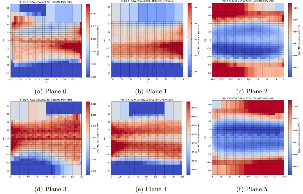
Figure 11: XTXZW data/MC MPV ratio maps for all planes.
