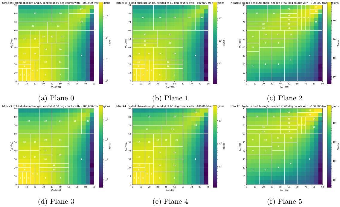
Figure 3: Folded 2D angular track distributions and selected WireMod angular regions. The angular plane is folded into (|\theta_{xw}|, |\theta_{yz}|) and the adaptive binning prioritizes the high-angle regions above approximately 60^\circ .
