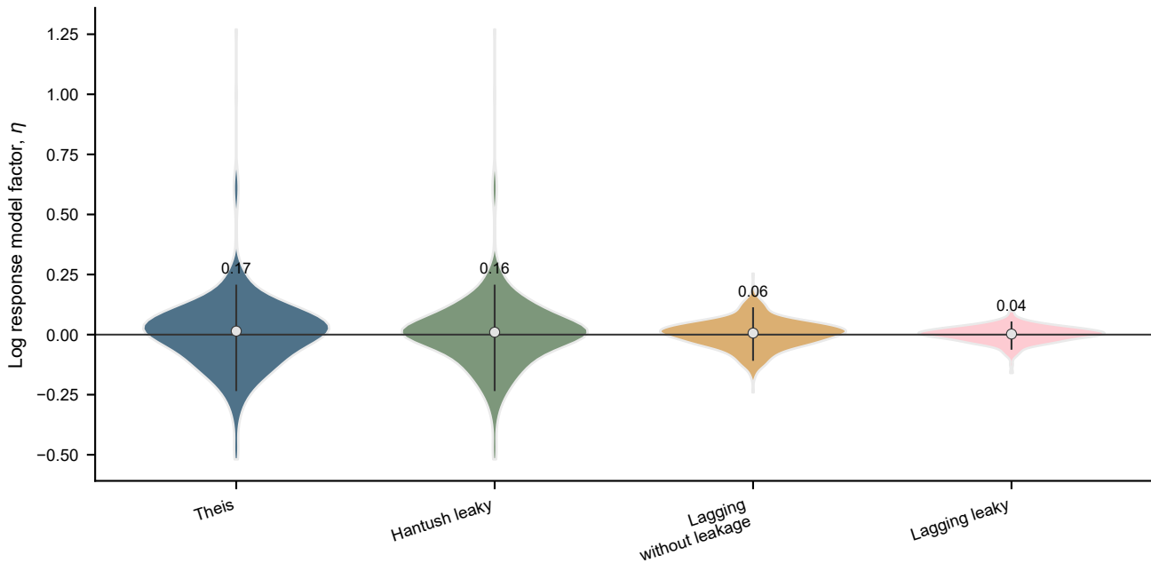
Pooled response residual distributions; numbers show pooled SD_{\epsilon}
