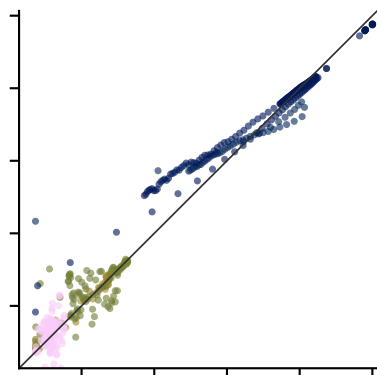
(b) Hantush leaky SD=0.294
