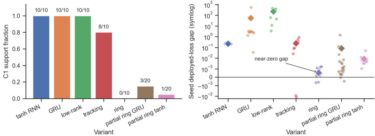
Figure 6: Generalization results across architecture and task variants. Standard variants use n = 10 paired seeds; the harder partial-observation ring variants use n = 20 paired seeds. Left: C1 support fractions with exact seed counts. Right: seed-level deployed-loss gaps with mean diamonds on a symmetric-log scale, which permits tiny or negative gaps while still showing large architecture gaps. C1 transfers to tanh RNN, GRU, and low-rank variants, is partial on tracking, and is weak or absent in ring path-integration variants.
