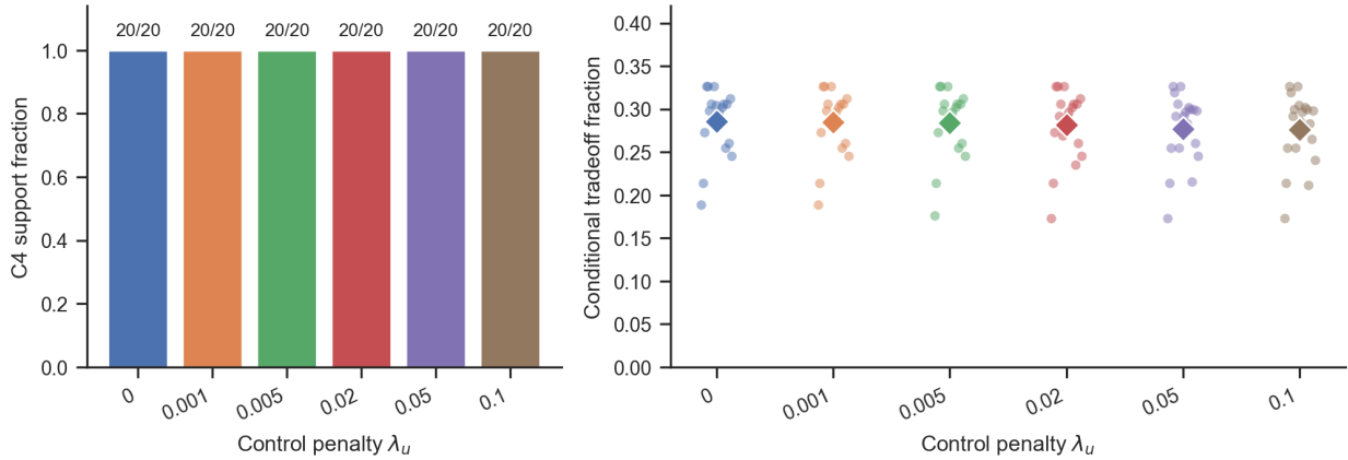
Figure 4: Targeted C4 short-vs-long horizon tradeoff sweep. Each condition uses 20 paired seeds. Left: all control-penalty settings support the predefined multi-horizon tradeoff criterion. Right: seed-level conditional tradeoff fractions, defined as the fraction of short-horizon improvement intervals that also show long-horizon worsening or increased coupled spectral radius. Diamonds show condition means.
