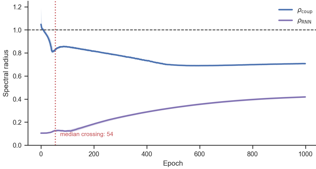
Figure 5: Coupled-system spectral analysis for the original setting. The coupled spectral radius crosses below the stability boundary early in training, whereas the RNN-only spectral radius remains far from the relevant stability threshold. This supports the original mechanistic claim that the coupled agent-environment system is the appropriate object of analysis.
