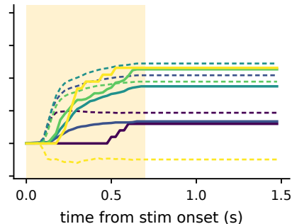
mouse 101 \Delta R^2=+0.50
