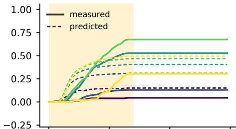
mouse 98 \Delta R^2=+0.66
