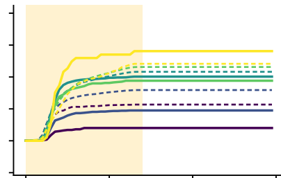
mouse 101 \Delta R^2=+0.50
