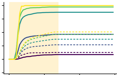
mouse 100 \Delta R^2=+0.20
