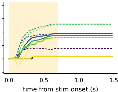
mouse 100 \Delta R^2=+0.20
