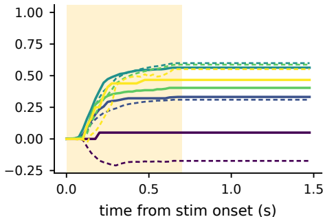
mouse 98 \Delta R^2=+0.66
