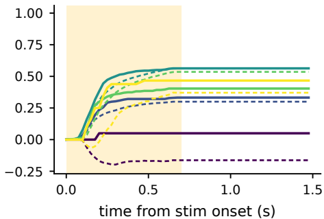
mouse 98 \Delta R^2=+0.70
