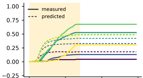
mouse 98 \Delta R^2=+0.70
