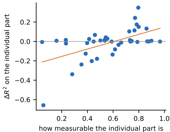
what transfers versus what is measurable rank correlation +0.44, p = 0.005
