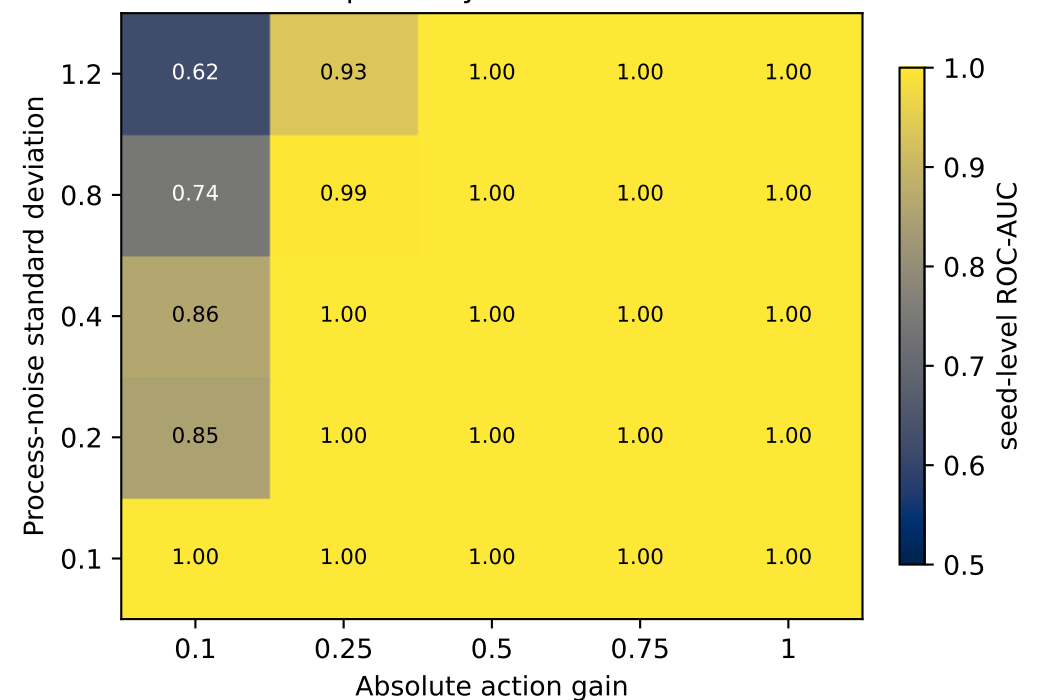
Coupled-vs-yoked ROC-AUC
