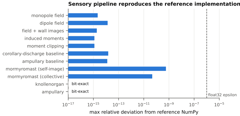
Figure 7: Maximum relative deviation from the reference NumPy implementation over random scenes, in double precision. Bars at the left edge are exactly zero.
