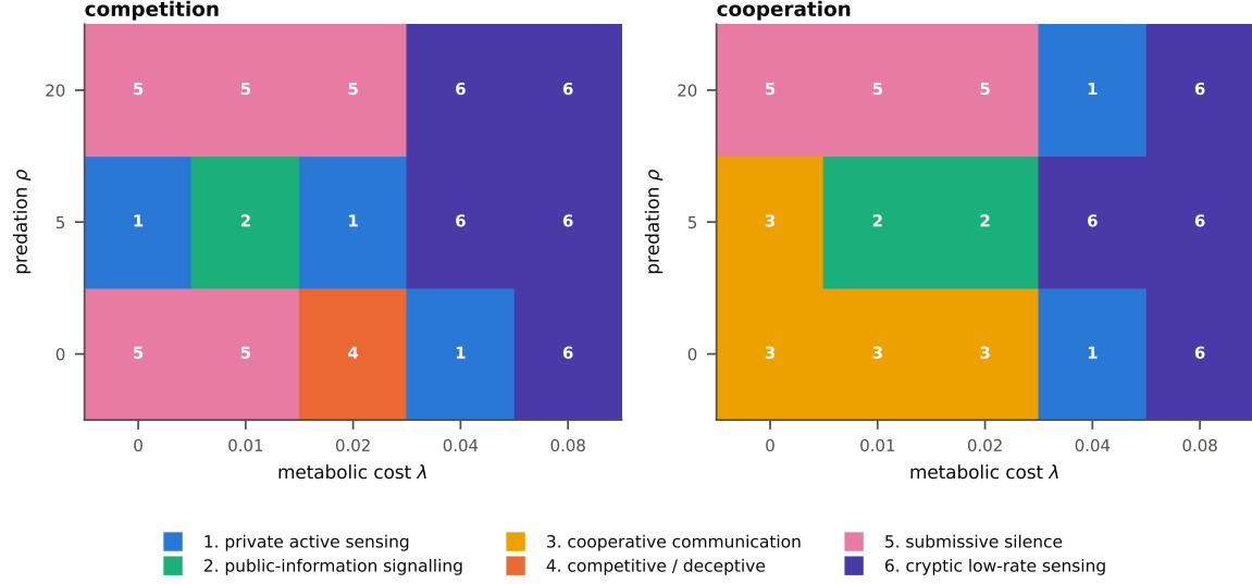
Figure 10: Rule-based regime labels from the pooled metric vector. Thresholds are percentiles of each metric’s own distribution across the grid rather than hand-set values, so the boundaries describe a continuum and are not claims about sharp transitions.
