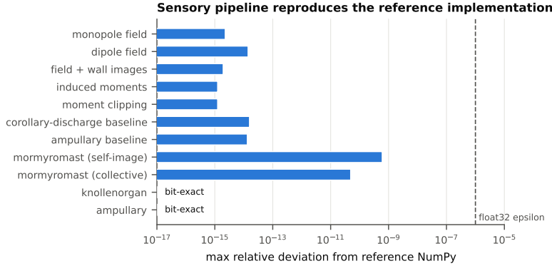
Figure 6: Maximum relative deviation from the reference NumPy implementation over random scenes, in double precision. Bars at the left edge are exactly zero.
