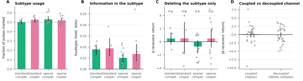
Figure 11: A discharge subtype decoupled from sensing, crossed with competitive and cooperative harvests and with a sparse-patch task in which finding food is the bottleneck. (C) deletes the subtype while leaving the pulse, and therefore all sensing, completely intact — the manipulation the coupled channel does not admit.
