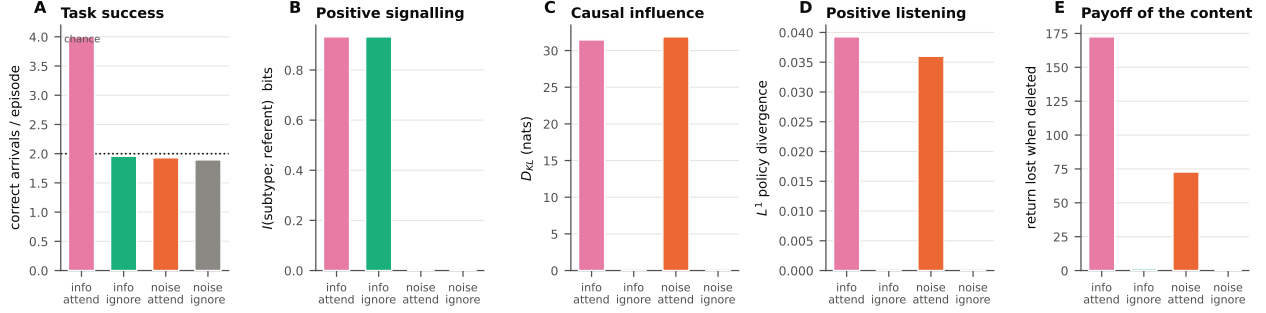
Figure 1: The assays detect communication when it is present, and each is foolable alone. Four dyads in the referential game. Only info+attend is communicating; the other three each satisfy some subset of the diagnostics.
