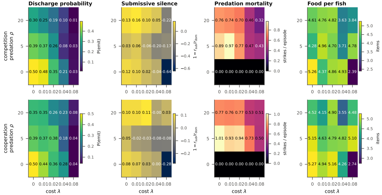
Figure 8: Metabolic cost and eavesdropping predation jointly set discharge policy. Rows are competitive and cooperative harvests; each cell is a mean over independent seeds.
