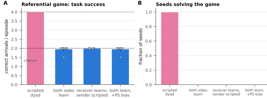
Figure 10: A hand-coded dyad solves the referential game from the same observations; twelve seeds each of three learned configurations, including one with a published bias designed for this problem, do not leave chance.
