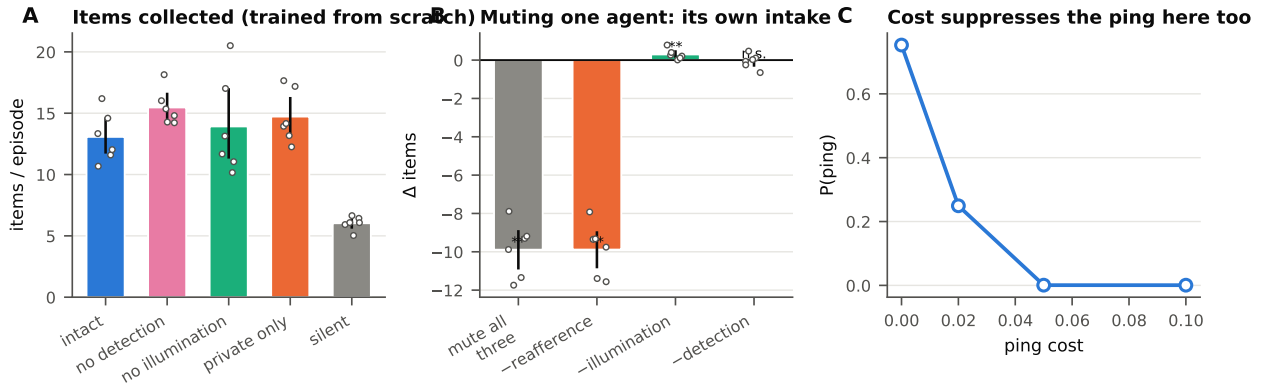
Figure 12: A minimal dual-use foraging world with no fish physics: a PING senses, illuminates neighbours and is registered as an event. The muting effect decomposes the same way as in the electric-fish environment, and cost suppresses the ping the same way.
