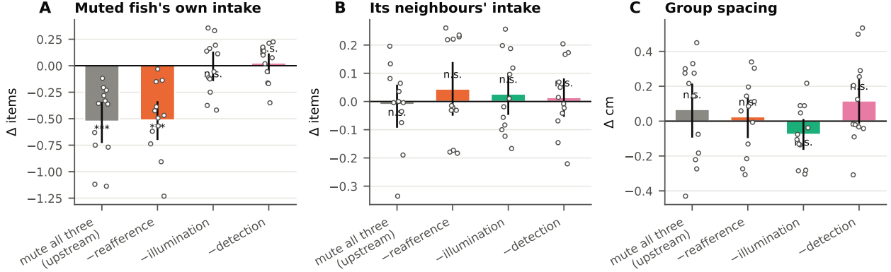
Figure 2: Silencing one fish removes three things at once; separating them reassigns the effect. Within-arena paired differences from the intact channel, frozen policies. Significance is a permutation test over seeds.
