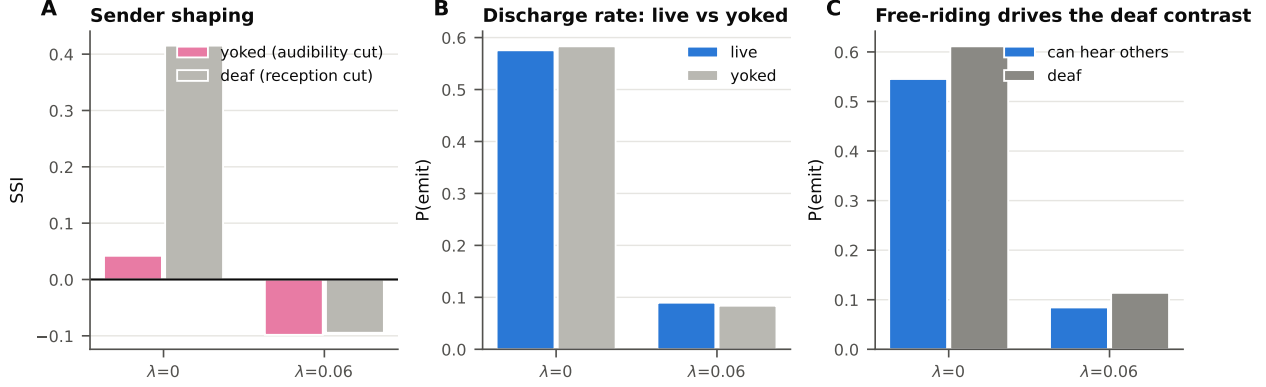
Figure 5: Sender shaping measured with reception held fixed. (A) SSI from the yoked contrast, which cuts audibility only, beside the confounded deaf contrast, which cuts reception. (B) Discharge rate, live versus yoked. (C) The free-riding effect that drives the deaf contrast: fish that can hear neighbours discharge less.
