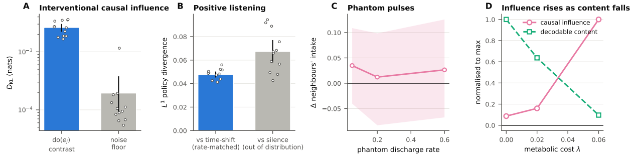
Figure 4: Positive listening, and why it is not enough. (A) Interventional causal influence against its noise floor (log scale). (B) Positive listening against a rate-matched time-shift null and against silence, which is out of distribution. (C) Phantom-pulse dose-response on neighbours' intake. (D) The dissociation: as metabolic cost rises, causal influence per discharge increases while the information a receiver can decode falls . Influence and informativeness move in opposite directions, so neither substitutes for the other.
