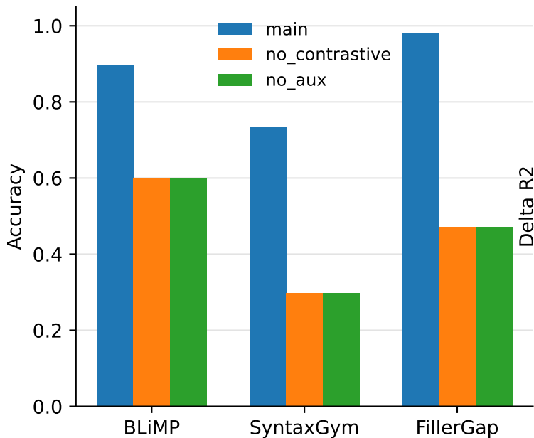
Auxiliary Training Carries Syntax/Filler
