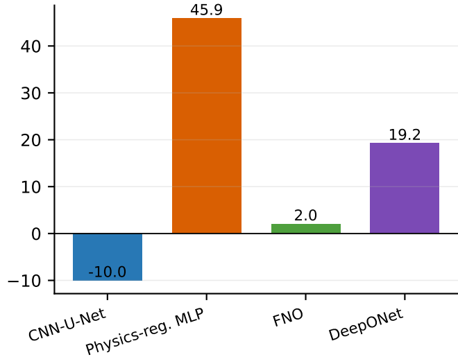
CFD-validated improvement (%)
