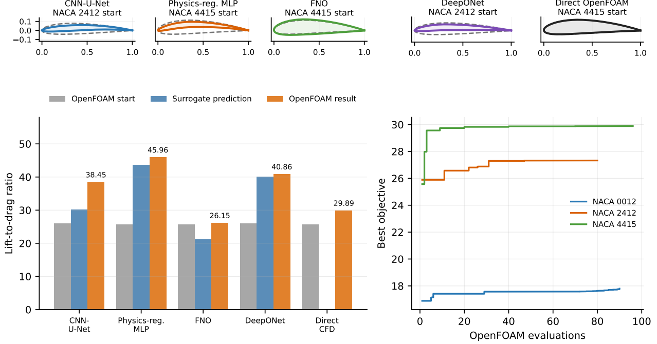
Fig. 5. Top: starting foils (dashed) and selected shapes. Bottom left: surrogate predictions, CFD endpoint checks, and the direct-CFD result. Bottom right: best-so-far objective during each direct OpenFOAM search.
