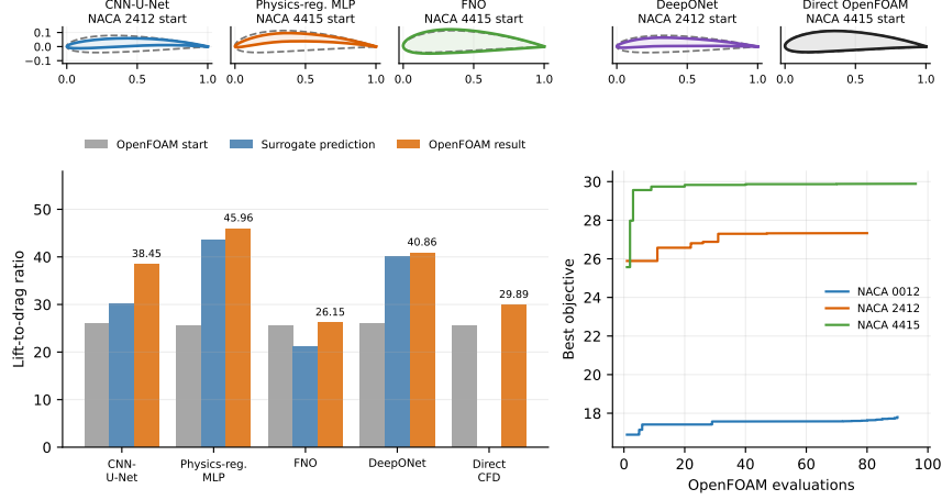
Figure 2: Top: starts (dashed) and selected shapes. Bottom left: surrogate predictions, CFD endpoint checks, and direct CFD. Bottom right: direct-CFD convergence from all three starts.
