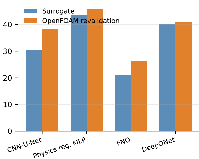
Lift-to-drag ratio
