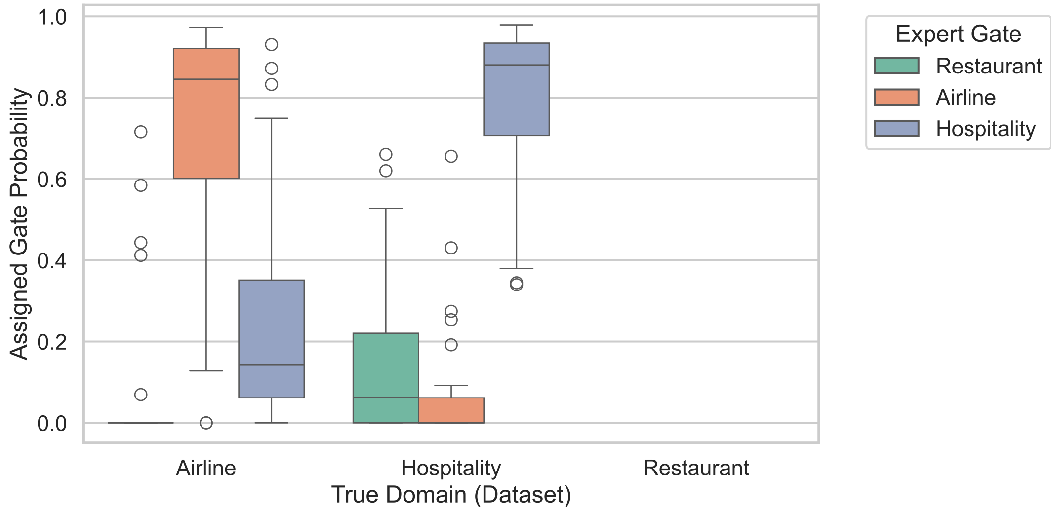
Fig 6: X-LoRA Gate Probability Separation
