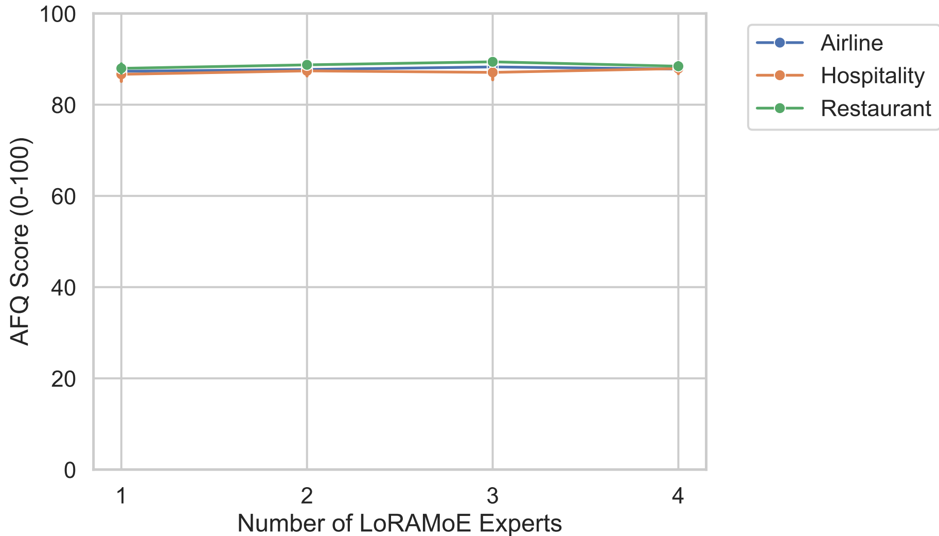
Fig 3: Emergent Expert Count Sweep
