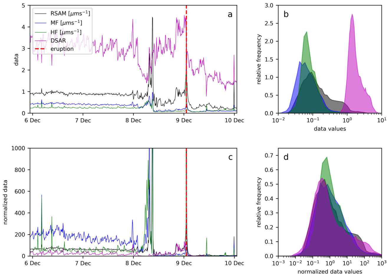
Fig. 5 Input data normalization. a Data time series prior and following the 2019 eruption (red dashed line): RSAM (black), MF (blue), HF (green), DSAR (magenta). b Histogram distributions of all data
