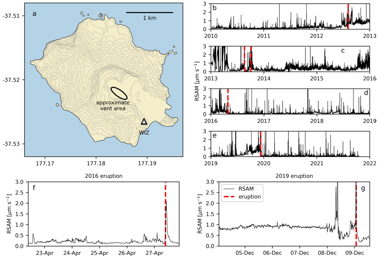
Fig. 1 Summary of tremor at Whakaari. a Map of Whakaari showing the location of the seismic station used in this study (white triangle) and the approximate vent area (Kilgour et al., 2021). Topographic contours have 20-m spacing, rising to approximately 300 m at the crater rim. b–e Real-time seismic amplitude measurement (RSAM)
