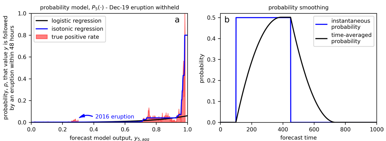
Fig. 9 Probability calibration and averaging. a Proportion of model outputs in y_{5,\text{agg}} followed 48 h later by an eruption (red). Fitted logistic/sigmoid (black) and isotonic regression (blue) models. b Time-averaging of instantaneous probability, in this case, a rectangular
