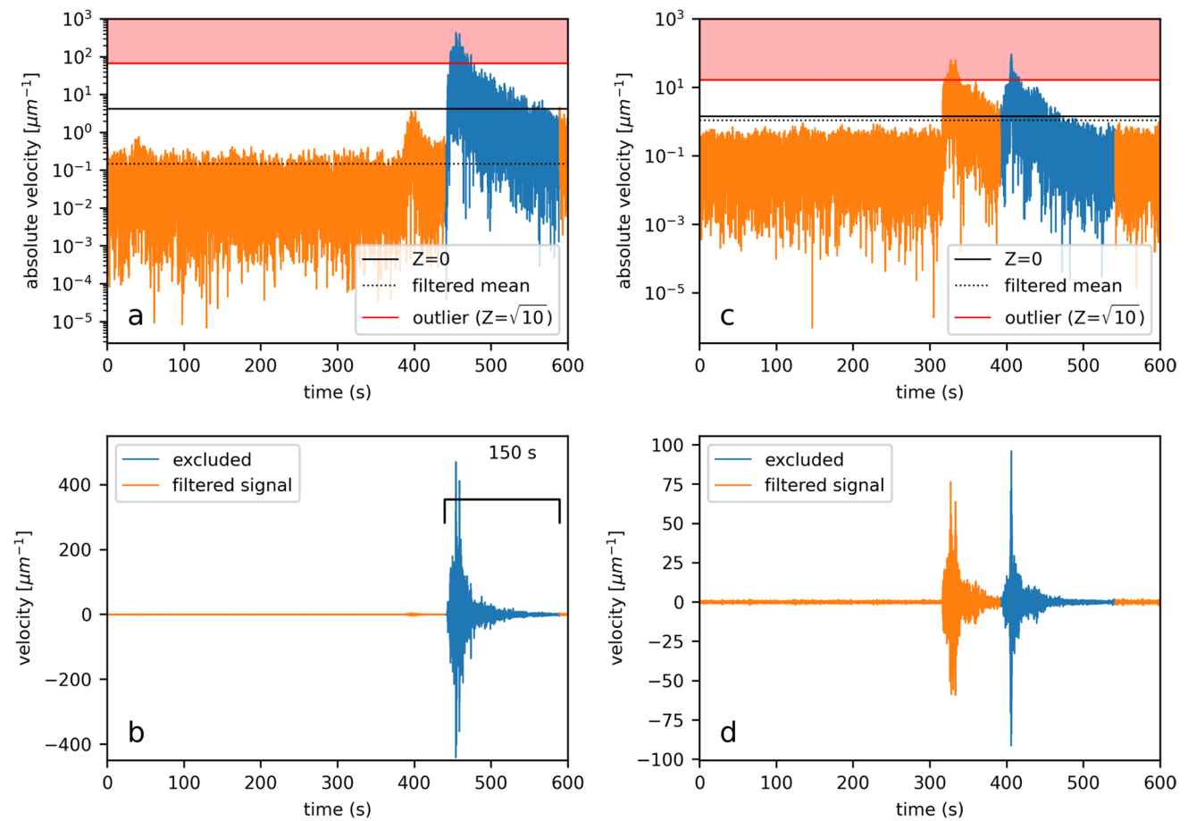
Fig. 4 Earthquake filtering during real-time seismic amplitude measurement (RSAM) calculation. a Absolute velocity time series on a log-scale showing the raw average (unfiltered RSAM, black line — a constant because it is an average over the 10-min data segment), a z -score threshold for outlier detection (red line) which was selected as \sqrt{10} \approx 3.2 , portion of the time series selected by the mask (blue) and the average (black dotted line) of the remaining time series (orange).
