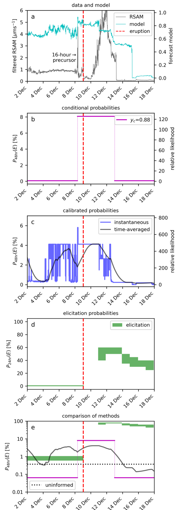
Fig. 10 Probabilistic forecasting of the December 2019 Whakaari eruption. a Tremor (black) and a time series of improved pseudo-prospective forecast model (cyan) prior to and following the eruption (red dashed). b Pseudo-prospective probability of eruption in 48 h calculated using a conditional probability model (Fig. 8) for a y_c=0.88 value to trigger a warning. c Pseudo-prospective probability of eruption in 48 h calculated using a calibrated probability model (Fig. 9). Blue=instantaneous, black=time-averaged probability. d Prospective probability of eruption in 24 h assessed by expert elicitation. Note, values prior to the December 2019 eruption have been converted from a 4-week forecast. e Comparison of the three probabilistic forecasts, where elicitation values have been converted to equivalent 48-h windows. The probability of eruption by an uninformed model is also shown (0.37% in 48 h, black dotted line)
