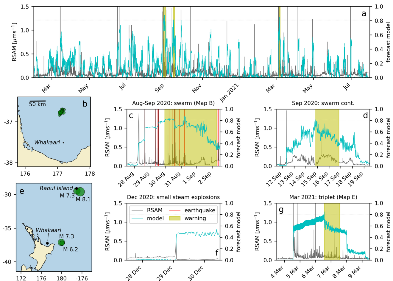
Fig. 3 Evaluation of an eruption forecasting system at Whakaari volcano between February 2020 and August 2021. a Real-time seismic amplitude measurement (RSAM; black), Dempsey et al. (2020) forecast model output (cyan), warning trigger threshold (black dotted) and warnings (yellow blocks) across the evaluation period. Notable periods include c , d two false positives triggered by an August–September 2020, which was triggered by a low-level tremor that followed a signal spike on 12 September (Fig. 3d). The spike was from an M_W 4.8 earthquake that was a continuation of the swarm to the north earlier that month (Fig. 3b). The third false positive occurred in March 2021 in response to a triplet of large earthquakes on the Kermadec subduction zone (Fig. 3f). The first event ( M_W 7.3) east of New Zealand was followed hours later by two more, 900 km away ( M_W 7.3 and 8.1), near Raoul Island (Fig. 3e). Contamination of the tremor signal by shaking from these events and their aftershocks led to a false positive 48 h after the first quake. All three false positives would have been avoided if regional earthquake signatures had been removed in real time from the tremor signal. All three false positives were “anticipated” or at least not unexpected when they did occur. This is because the earthquakes did not immediately trigger the model, but rather started it on an upward trend over several hours, toward the trigger level. This provided time to confirm (by waveform
