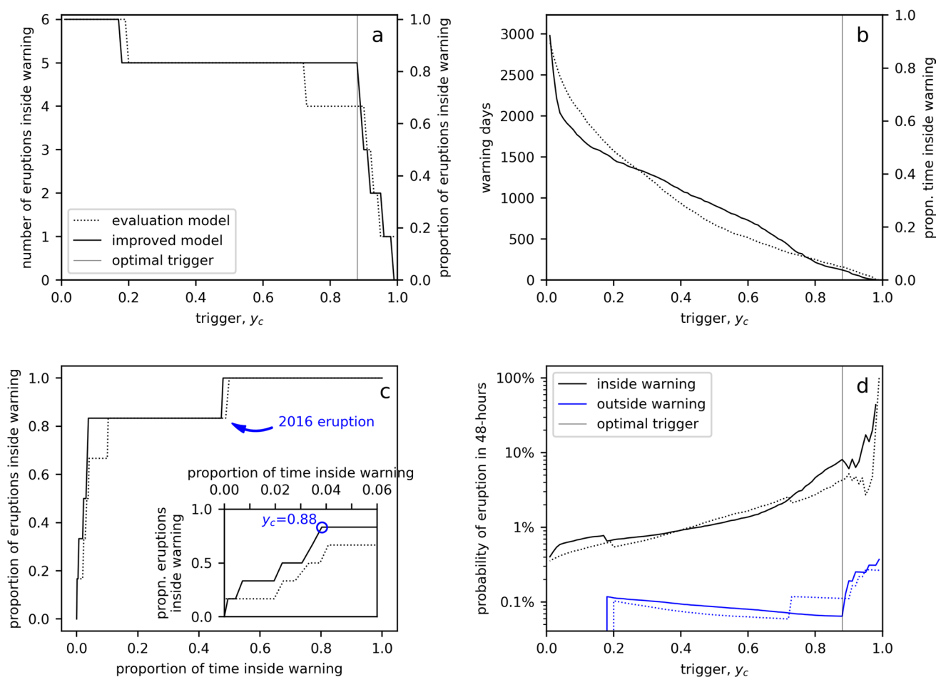
Fig. 8 Performance of two probabilistic warning systems trained using data prior to December 2019: the Dempsey et al. (2020) evaluation model (dotted), and the improved model with earthquake filtering, data normalization and retraining (solid). a Rate of missed eruptions for different warning triggers, y_c . b Total duration of all warnings, out of a maximum possible 3234 days. Panels a and b
