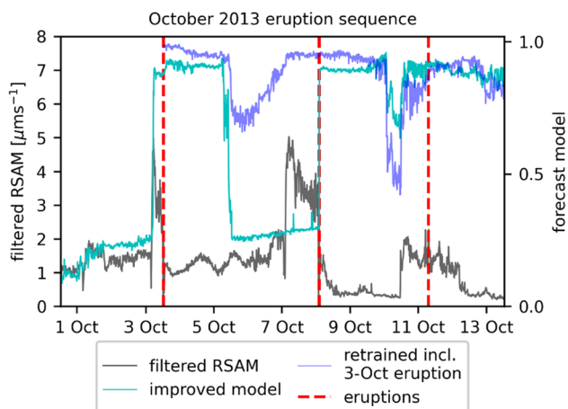
Fig. 6 Effect of model retraining on forecast performance during an eruptive sequence. Here, a pre-trained model (cyan) detects two out of three eruptions in a sequence. When the model is retrained after the first eruption using the recently acquired data, all subsequent eruptions are anticipated at high confidence
