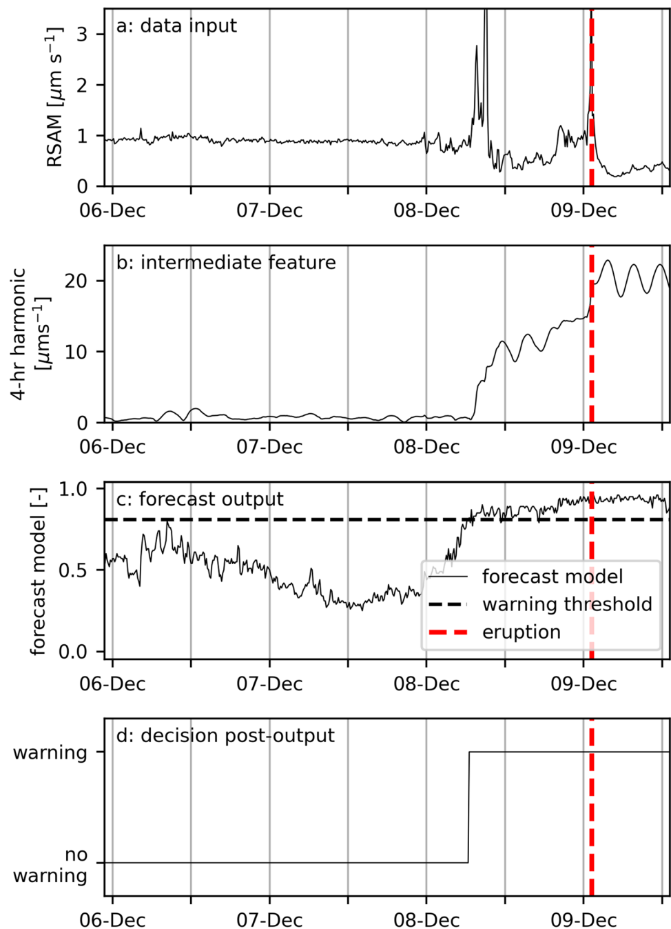
Fig. 2 Time series feature engineering as the basis of an eruption forecast model. a Real-time seismic amplitude measurement (RSAM) time series prior to the 2019 eruption. b Example of a time series feature, in this case, the absolute value of the 4-h harmonic obtained from a fast Fourier transform applied to a sliding window over the RSAM record in a . The window is constructed from the 48 h of data prior to the feature date-time. c Output of the Dempsey et al. (2020) forecasting model, which combines many such time series features by means of a random forest classifier. d Example of a simple warning system, triggered when the model value in c exceeds a pre-determined threshold (black dashed line)
